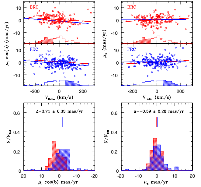
Fig. 6. Upper panels: PMs versus RVs for BRC and FRC sample. Color lines (red for BRC and blue for FRC) shows the linear regression for our data in the respective sample. As is shown in the right upper panel, no significant difference in \mu_b versus RV is observed, while for \mu_l \cos(b) a common trend with RV is found ( left upper panel ). Under each scatter plot is also shown the scaled RV distribution for each sample to define a pure BRC and FRC sample (red and blue dashed regions, respectively). Lower panels: histograms for observed proper motions and the difference in the median for selected stars in each pure sample defined above.
