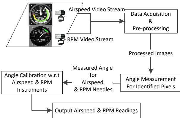
Figure 1. Framework for automated dial reading
