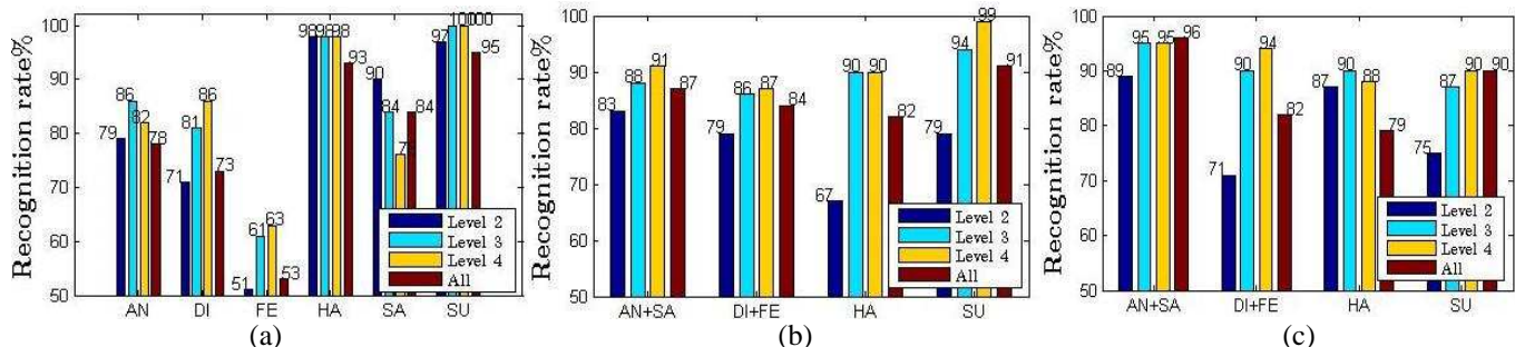
Figure 3. Recognition rate (%) for (a) the supervised method with 6 classes (b) supervised method with 4 classes, and (c) unsupervised method with 4 classes as a function of different expressions and different expressions' intensities.
