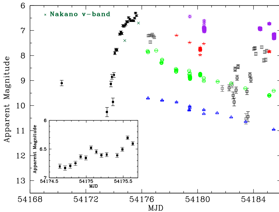
Figure 6. Optical light curves of V2467 Cyg indicating the peak of the nova and its initial decline. SMEI data with a lower r than optimal have been included for completeness. AAVSO data which coincide with the SMEI light curve have been included (see Figure 1 for data legend). The two green crosses represent data from Nakano et al. (2007a). The inset shows the final rise, peak, and initial decline of the nova in the SMEI data only.
