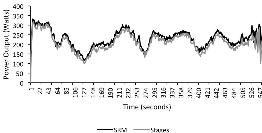
Figure 2. Power output averaged at 1 second intervals for SRM and Stages Powermeters.
