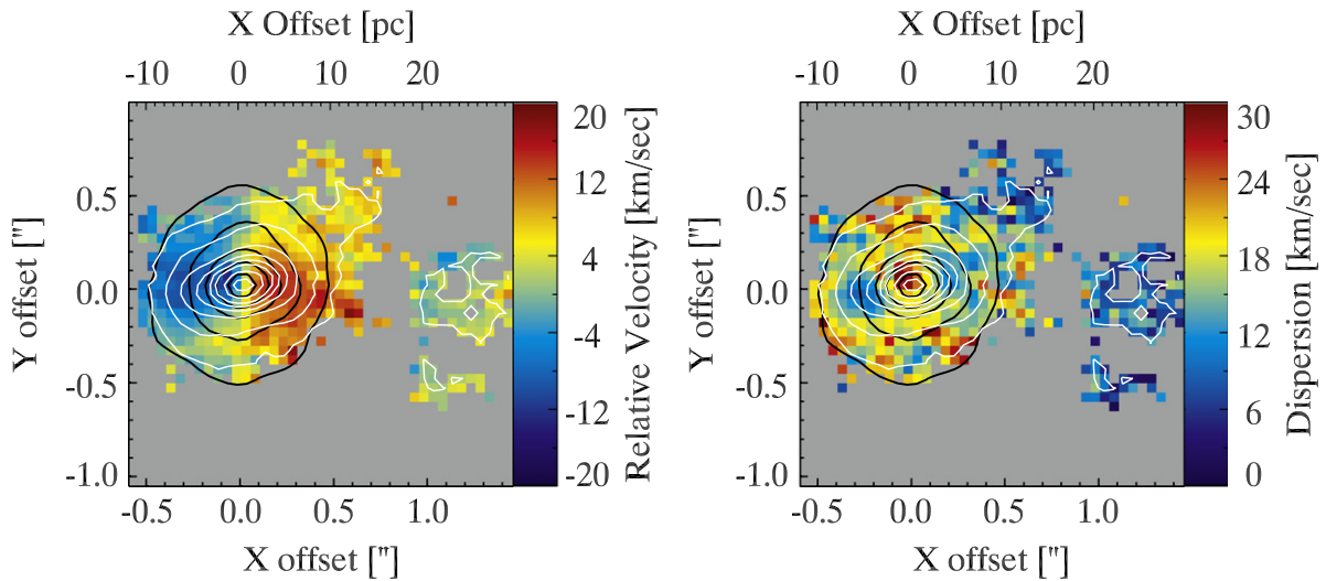
Figure 1. \text{H}_2 1–0 S(1) velocity and velocity dispersion fields. North is up, and east is left. White contours represent the intensity of the \text{H}_2 emission, and black contours represent the total intensity in the K_s band.
