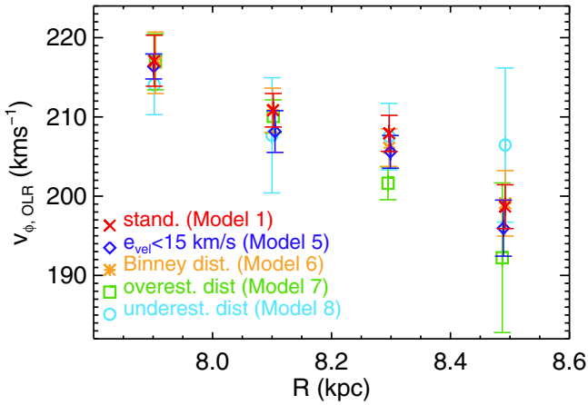
Fig. 15. Position of the v_{\phi, \text{OLR}} as a function of R for the band at \phi_b + 6 deg for different cases of RAVE data.
