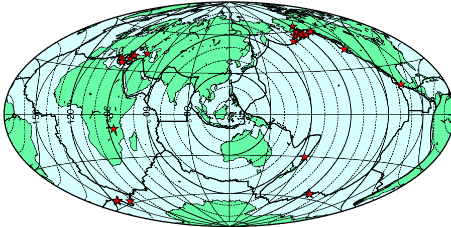
Figure 2. Teleseismic earthquakes (red) used in the SKS splitting analysis.
