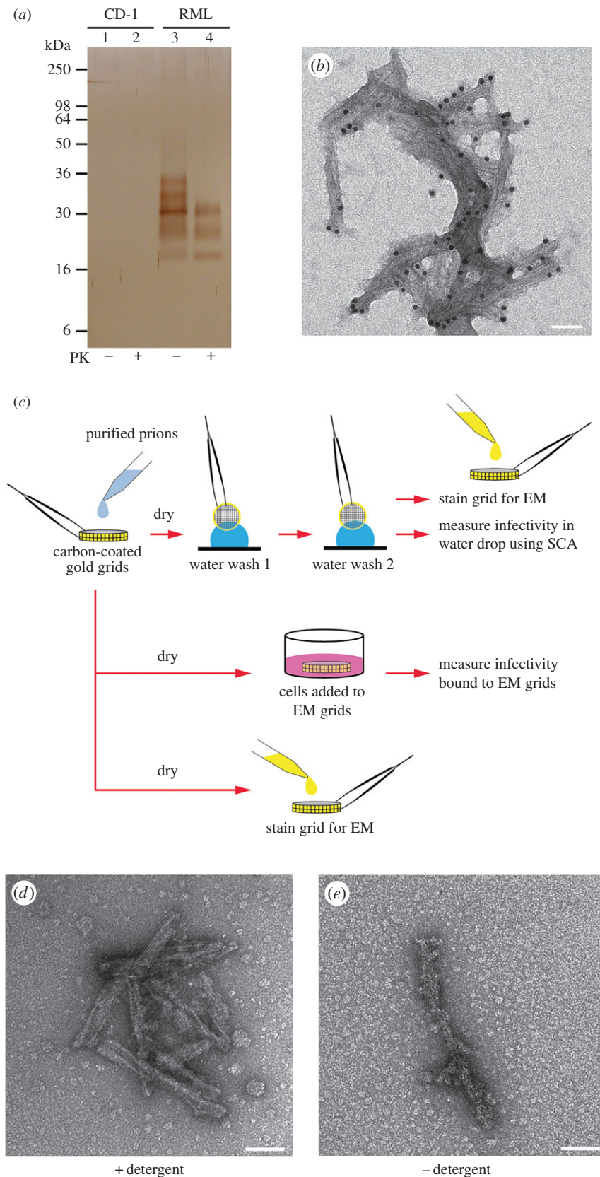
Figure 1. Ex vivo PrP rods are physically associated with prion infectivity. (a) Silver-stained 16% SDS-PAGE gel of RML prion preparations purified with (+) or without (-) proteinase K (PK) digestion compared to equivalent fractions from uninfected normal CD1 mouse brain. (b) EM image of an RML prion preparation purified without PK digestion. PrP rods (shown here immunogold-labelled with an anti-PrP monoclonal antibody) are the only visible protein structures. (c) Schematic of novel cell culture methods (Scrapie Cell Grid Assay, SCGA) used to measure prion infectivity bound to the surface of EM grids. (d) EM image of PrP rods (RML strain) observed when purified prion samples are dried onto the microscope grid without washing with water. Visible background objects are non-protein buffer artefacts (that include detergent micelles). Purified prions bind tightly to grids with less than 5% of the applied infectivity removed from dried grids by successive water washes; see the electronic supplementary material, table S1. The SCGA reported prion infectivity titre with an efficiency equivalent to, or better than, measuring prions in solution, see the electronic supplementary material, table S2. (e) EM image of PrP rods (RML prion strain) isolated from brain without the use of detergent. Scale bars, 50 nm.
