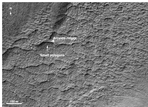
Figure 7. HiRISE observation showing a field of small arcuate depressions (image ID: ESP_015943_1390, image center: 40.5°S, 54.2°E). This view reveals the arcuate tops of the depressions and the small polygons observable on the floor of the depressions. Here the arcuate depressions cover a range of different elevations.
