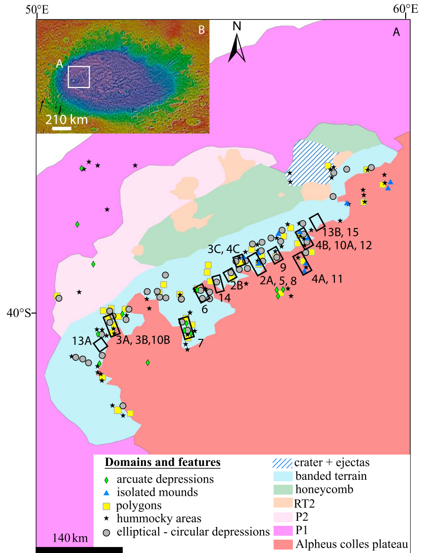
Figure 1. (A) Geomorphologic map of the NW Hellas basin showing the different domains and the location of the ice-related landforms and (B) insight of a general Time History of Events and Macroscale Interactions during Substorms day IR map overlaid with MOLA color elevation map of Hellas to present the location of the study area (white box on the B). The colored areas on the map (A) represent the different domains and the color symbols show the landforms for clarity. Colored areas are: the Alpheus Colles plateau (red), a local crater with its ejecta (dashed blue), the plain deposit 1 (P1; dashed black), the plain deposit 2 (P2; pink), the honeycomb terrain (green), the reticulate terrain 2 (RT2; maroon), and the banded terrain (light blue). Colored symbols are arcuate depressions (green diamonds), isolated mounds (blue triangles), polygons (yellow squares), hummocky areas (violet stars), and elliptical to circular depressions (red dots). The black boxes associated with black numbers indicate the location of the other figures of the paper.
