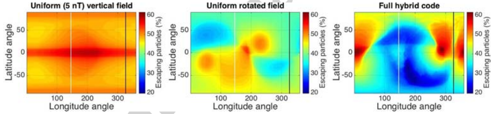
Figure 8: Access of 10 keV H^+ ions to Titan's exobase for the case of a uniform vertical field (left), a rotated uniform field (centre) and the full hybrid code output (right). The white vertical line indicates the position of the ram direction while the black vertical line indicates the position of the tail.
