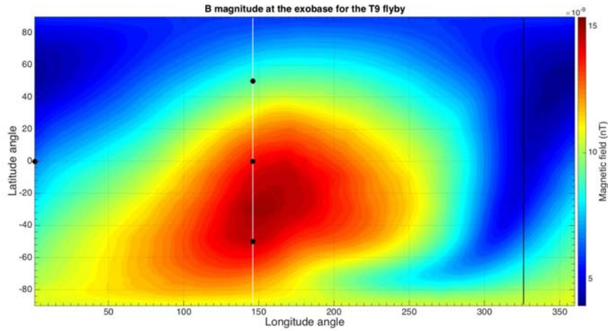
Figure 11: Magnetic field magnitude for the T9 flyby at Titan's exobase as obtained from a hybrid code (A.I.K.E.F.) simulation. The white vertical line indicates the position of the ram direction while the black vertical line indicates the position of the tail. At the position of the ram direction, a pile up of the magnetic field lines enhances the magnetic field magnitude whereas a depletion of magnetic field lines can be observed on the tail, where the magnetic field magnitude is around 3 times smaller. This affects the access of particles with small gyroradii, allowing them to access regions close to the tail while preventing them to access regions close to the ram direction. The four black markers indicate the regions at which ionization rates are calculated (see later sections in the paper).
