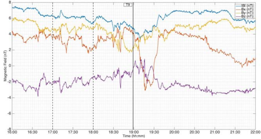
Figure 13: Magnetic field data in TIIS coordinates three hours before and after closest approach (marked here with the solid black line in the middle of the plot) for T9. The dashed lines show the region of undisturbed magnetic field from which the ion data used in the analysis were taken.
