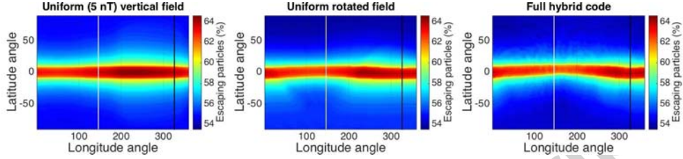
Figure 7: Access of 10 keV O^+ ions to Titan's exobase for the case of a uniform vertical field (left), a rotated uniform field (centre) and the full hybrid code output (right). The white vertical line indicates the position of the ram direction while the black vertical line indicates the position of the tail.
