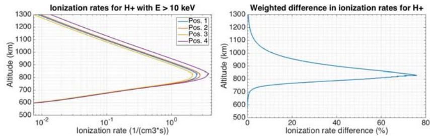
Figure 17: Production rates from precipitating H^+ ions with energies higher than 10 keV (left panel) at four different positions around the moon and weighted difference between the positions with higher (position 4) and lower (position 3) rates.
