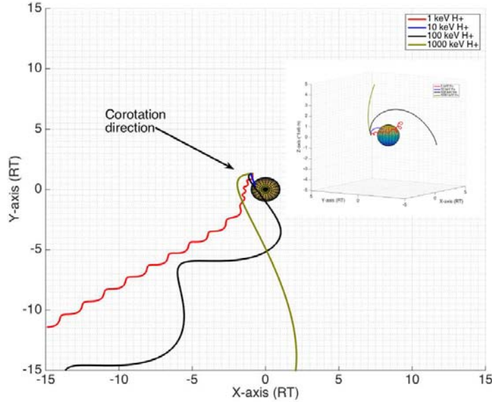
Figure 2: Trajectories of four different H^+ ions starting at the same initial position. All the ions were simulated with the same starting polar and azimuthal angles, the only difference being their starting energy. The difference in gyroradius that is induced by this difference in starting energies leads to completely different trajectories, with 10 keV ion colliding with the moon soon after starting the simulation while the others finally escape the interaction region.
