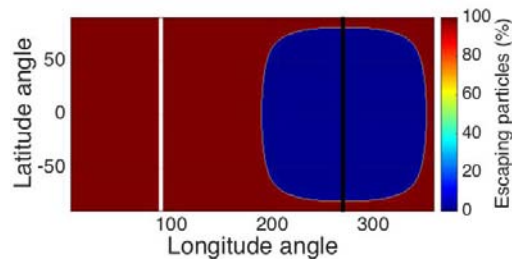
Figure 3: Equirectangular projection of Titan's exobase showing the access of 1 keV electrons for an ideal north-south field configuration. The white vertical line indicates the position of the ram direction while the black vertical line indicates the position of the tail. Due to the uniform nature of the magnetic field configuration used and the lack of parallel velocity of the propagated particles, a large depletion in the access of particles is observed on the tail of the moon. Small areas on the tail where particles can access are present since the lower boundary of the simulation is taken 50 km below the defined exobase (see text for further explanation).
