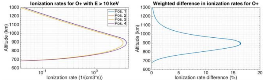
Figure 16: Production rates from precipitating O^+ ions with energies higher than 10 keV (left panel) at four different positions around the moon and weighted difference between the positions with higher (position 4) and lower (position 3) rates.
