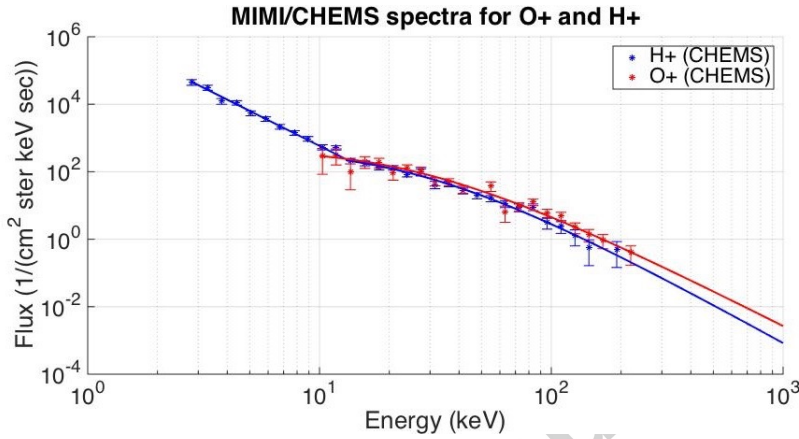
Figure 14: MIMI/CHEMS spectra for O^+ and H^+ ions during the T9 flyby. The oxygen spectrum (red curve) was fitted with a Kappa distribution while the hydrogen spectrum (blue curve) was fitted with a power law for the lower energies and a Kappa distribution for the higher energies. Both spectra were extended with the fitted curve until 1 MeV.
