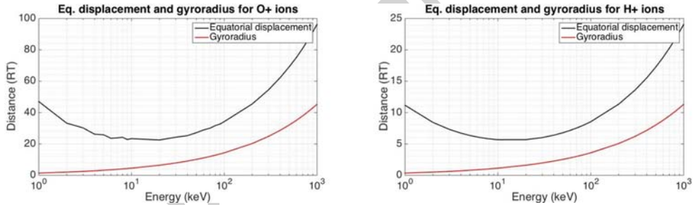
Figure 6: Half-bounce averaged equatorial displacement and gyroradius for O^+ and H^+ ions at different energies.
