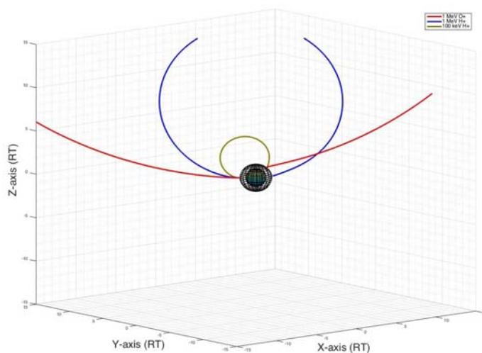
Figure 4: Example of particles with gyroradii larger than the moon colliding after one gyration. All the three particles shown in the plot reached a region of undisturbed electromagnetic field upstream of the moon but, due to their large gyroradii, returned to the interaction region after one gyration and finally collided with the moon's exobase (shown as the black grid surrounding the moon in the center of the figure). Notice that the choice of the inner boundary (the black grid) could affect the access maps presented in the results section, with for instance the particle with the red trajectory possibly escaping the system if the boundary were set at a lower altitude. This effect is analyzed in the Appendix A.
