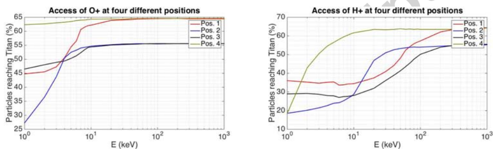
Figure 12: Percentual access of O^+ and H^+ ions vs. Energy at four different locations in Titan's exobase.
