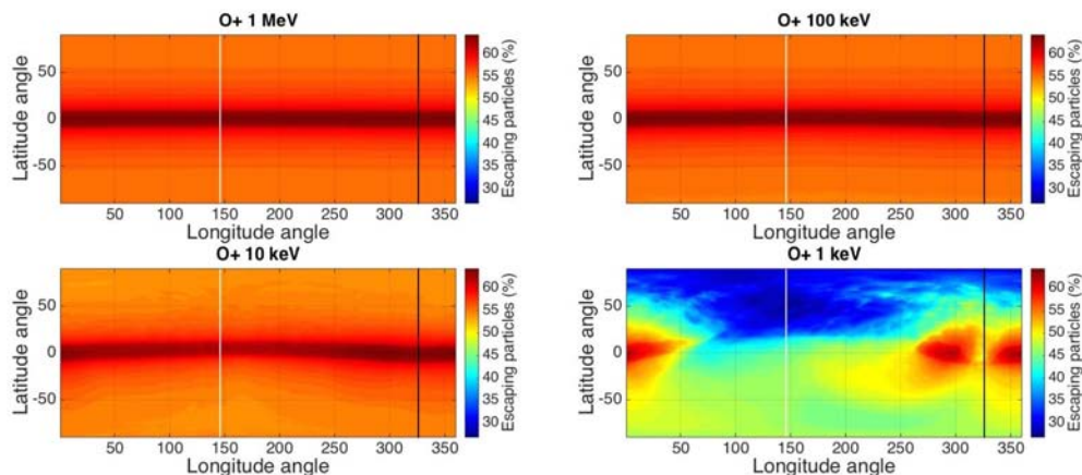
Figure 9: Equirectangular projection of Titan's exobase showing the access of 1 MeV (top left), 100 keV (top right), 10 keV (bottom left) and 1 keV (bottom right) O^+ ions. The maps were created by propagating the particles on a background electromagnetic field generated by the A.I.K.E.F. hybrid code. The white vertical line indicates the position of the ram direction while the black vertical line indicates the position of the tail.
