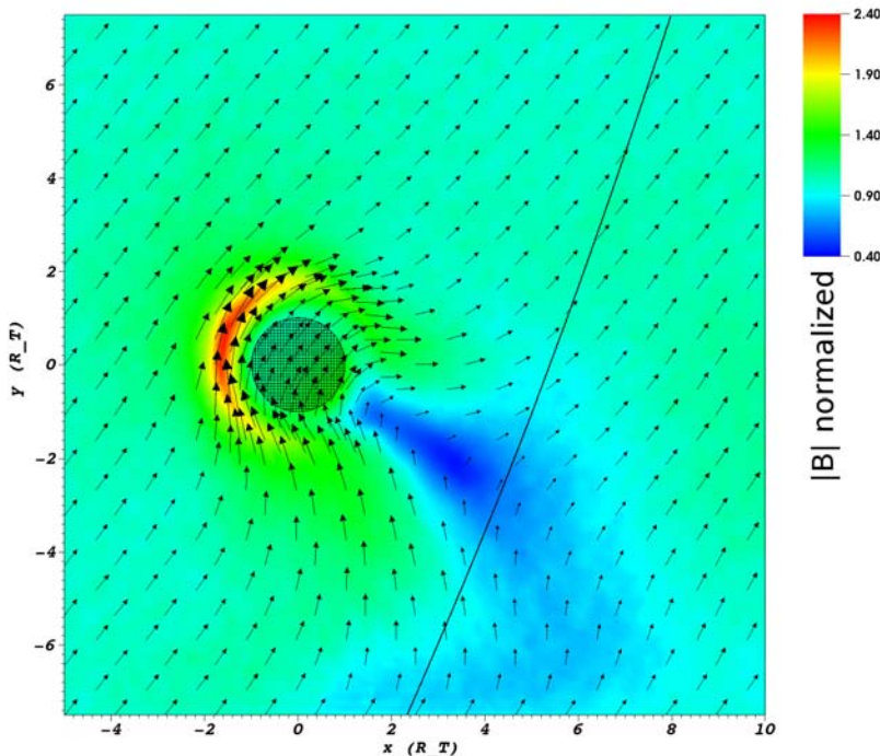
Figure 5: Equatorial magnetic field in TIIS coordinates within a simulation box of 15 R_T side during the T9 flyby as calculated using the hybrid code A.I.K.E.F. The colors represent the magnitude of the magnetic field normalized to the upstream field magnitude ( 6.37 \text{ nT} ) and the black line shows Cassini's trajectory during the flyby.
