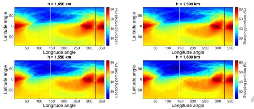
Figure A.18: Access of 1 keV O^+ ions to four different altitudes: 1450 km (exobase, top left), 1500 km (top right), 1550 km (bottom left) and 1600 km (bottom right).
