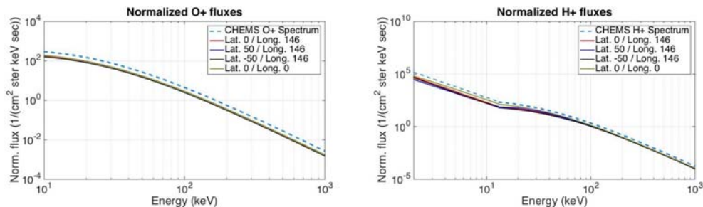
Figure 15: Normalized flux vs. Energy for O^+ and H^+ ions at four different locations in Titan's exobase. These fluxes are used as an input for the ionization rates shown in Figures 16 and 17.
