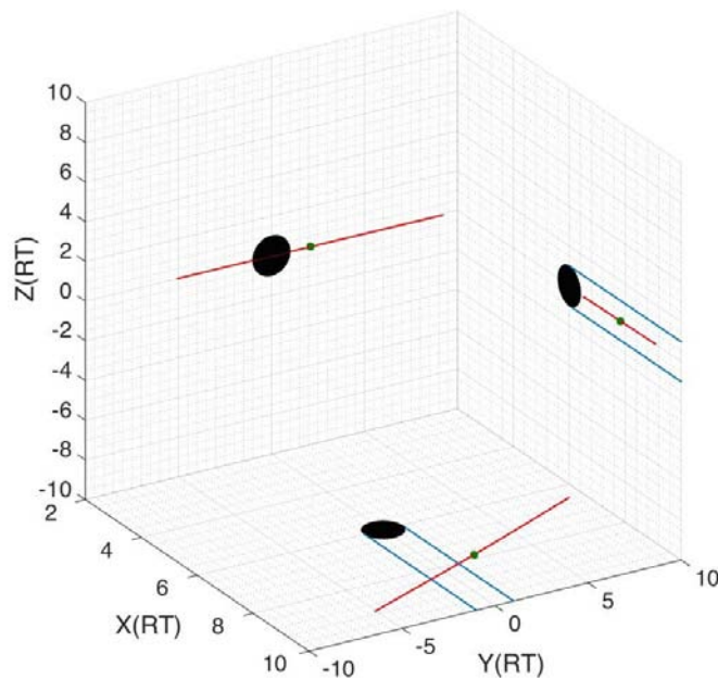
Figure 1: Cassini trajectory during the T9 flyby shown in the THIS coordinate frame. The X-axis points in the direction of ideal corotation, the Y-axis points towards Saturn and the z-axis points northwards. The red line represents the spacecraft trajectory with the green point in the middle representing the moment of closest approach. The ideal corotation tail is represented by the two parallel blue lines.
