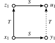
Figure 1: Completing the square with Boolean CQ \neg 1^S (3).
