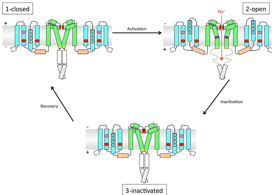
Figure 5. Schematic diagram of (1) closed, (2) open, and (3) inactivated states of prokaryotic sodium channels based on crystallographic studies. Only two monomers are shown in each figure for clarity. The color scheme is as in Fig. 1. The VS S1–S4 helices are depicted as cyan bars, the S4–S5 linker is an orange bar, the S5–S6 helices of the pore region are green bars, and the coiled-coil region of the CTD is gray. The extracellular negatively charged region in S2 is in a magenta circle, and the intracellular negatively charged regions in S2 and S3 are in red circles. The four arginines in S4 involved in the gating charge transfer across the membrane through sequential interactions, with the extracellular negatively charged region and the intracellular negatively charged region represented by a “+.” The residues forming the SF are indicated by red boxes. The residue in purple is the start of the S6 twist that results in the open gate; the residue in yellow is the third hydrophobic constriction site in the closed form, which is not constricted in the open form, and indicates the position of the activation gate. The white bars represent the helical region present in the CTD in the closed and inactivated structures, and the corresponding dotted gray lines are the disordered CTD linker region in the open conformation.
