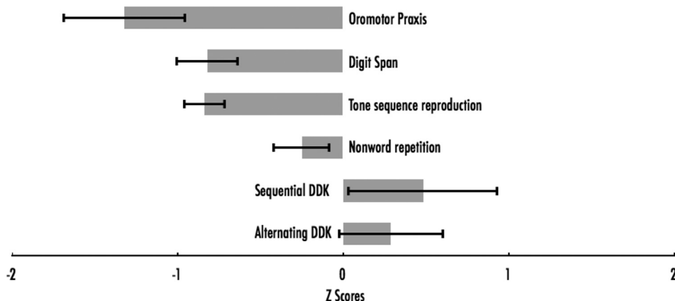
Fig. 3. Means and standard errors of z -scores. for the WS group relative to VSMA controls. Negative z -scores. indicate lower scores than the average of the VSMA group, whereas positive z -scores. suggest that scores are higher.
