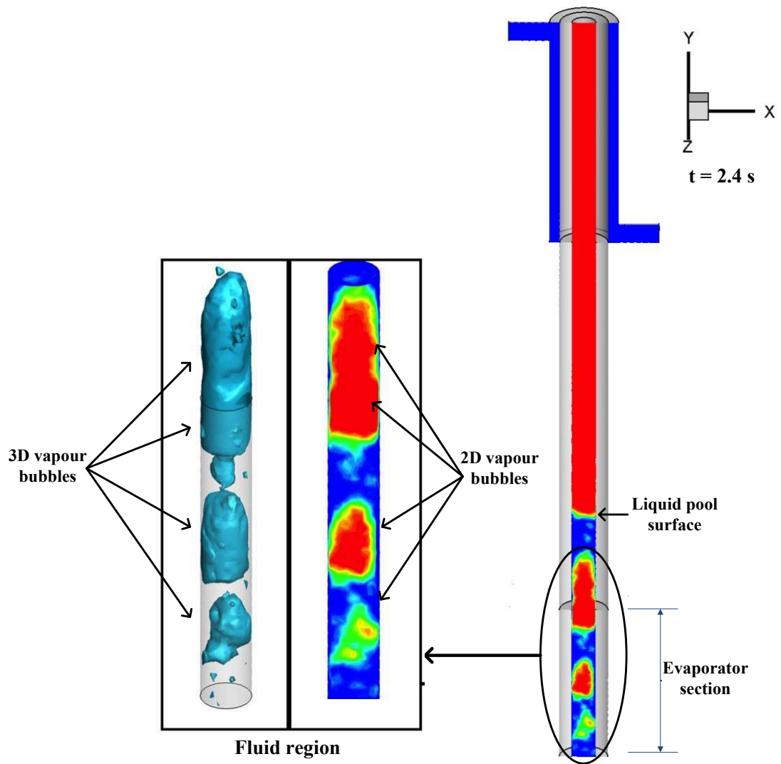
Figure 8: Size of the vapour bubbles in the evaporator section for a power throughput of 30W
