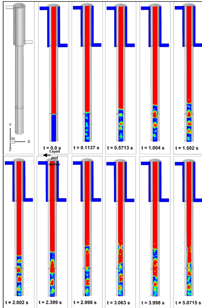
Figure 7: Geyser boiling process in a thermosyphon for a power throughput of 30W
