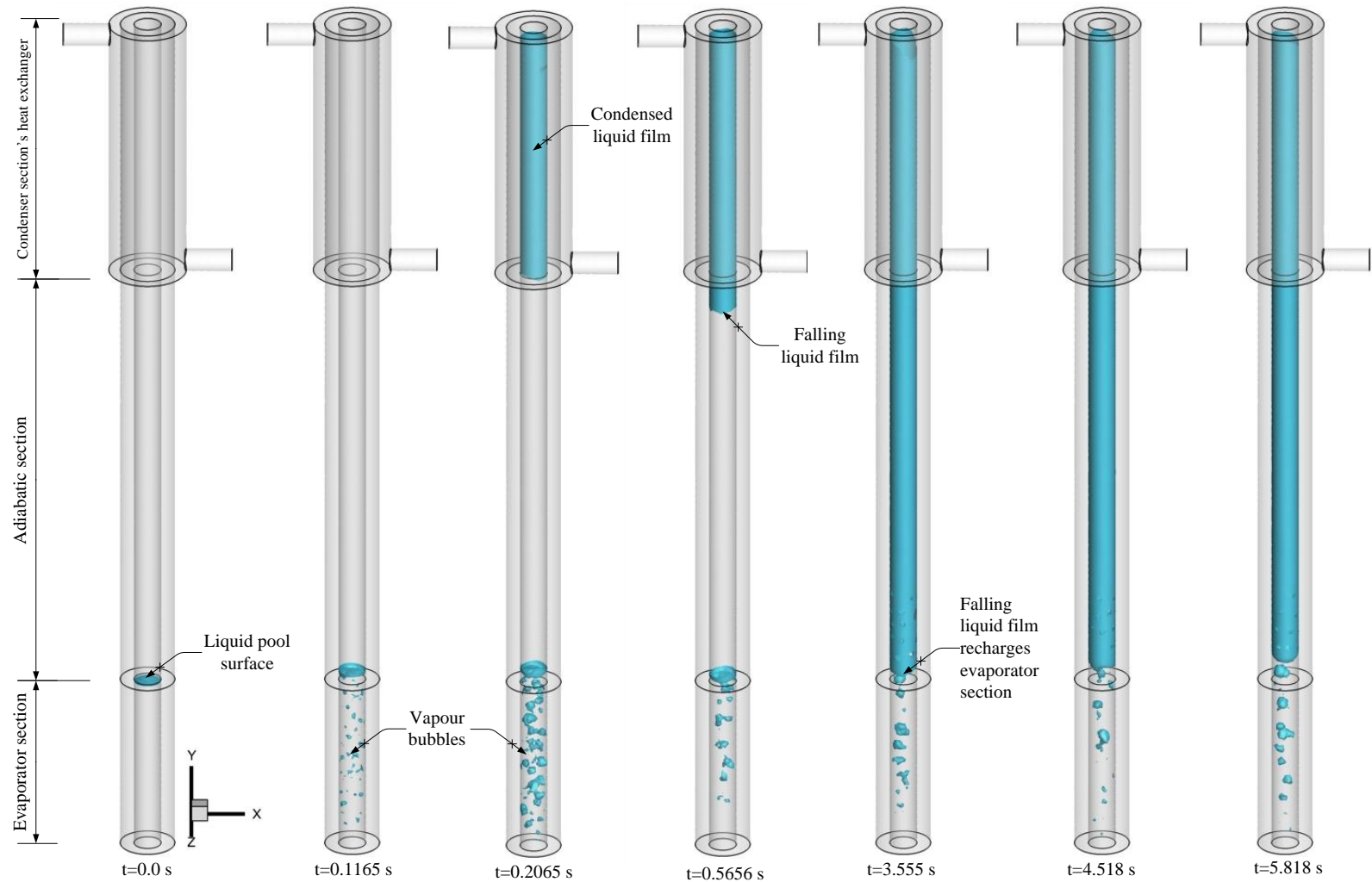
Figure14: Three-dimensional CFD modelling of evaporation and condensation for a thermosyphon charged with R134a for a power throughput of 30W
