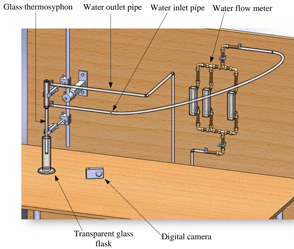
Figure 12: A glass thermosyphon experimental apparatus framework
