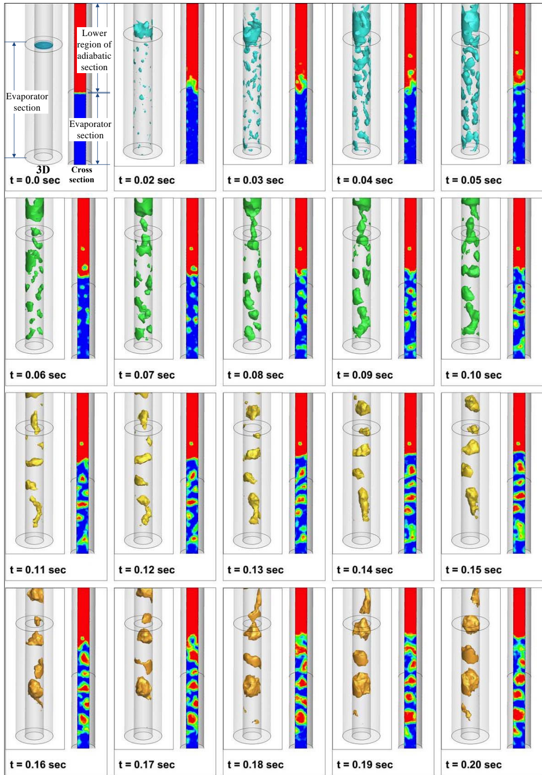
Figure 9: Pool boiling process in a thermosyphon for a power throughput of 220 W
