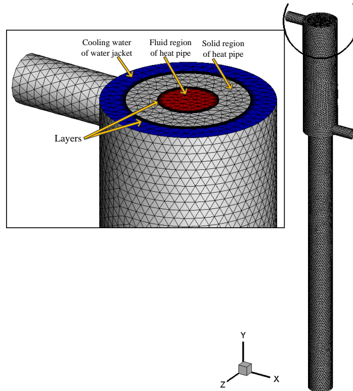
Figure 2: The computational mesh used in the simulation of a two-phase closed thermosyphon with water jacket
