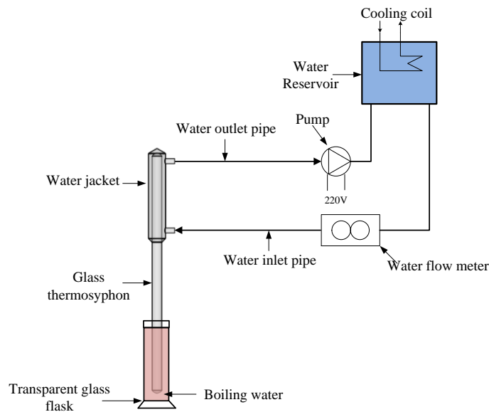
Figure 10: A glass thermosyphon experimental apparatus
