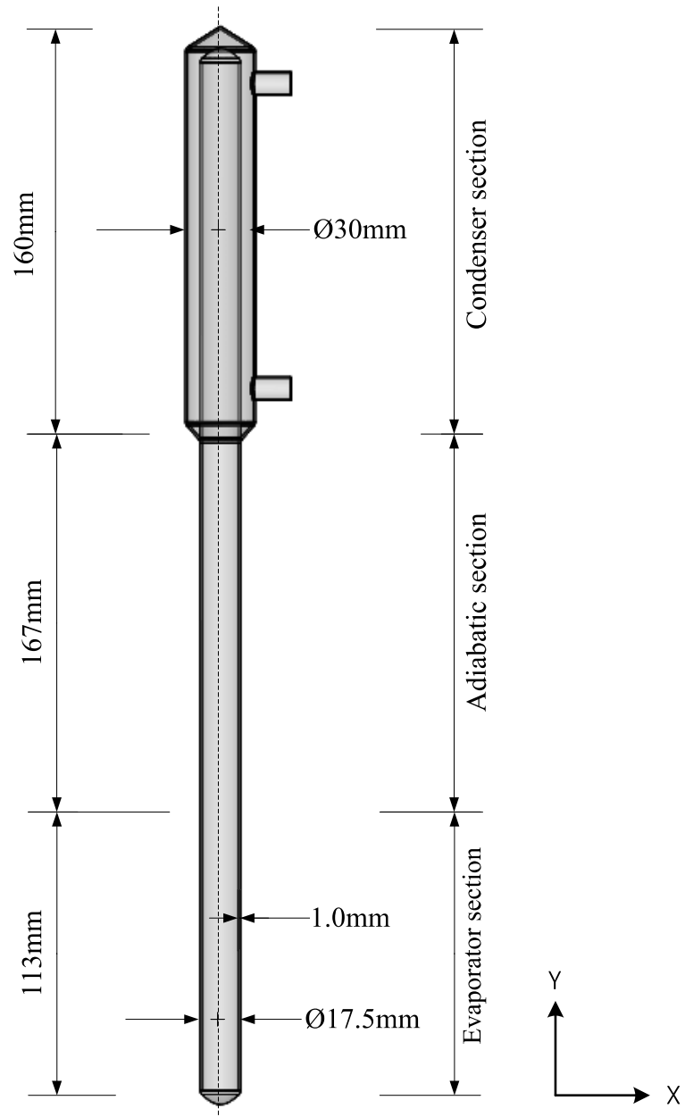
Figure 11: A transparent glass thermosyphon dimensions
