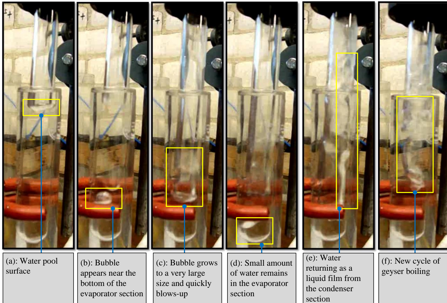
Figure 13: Visualisation of geyser boiling using transparent glass thermosyphon
