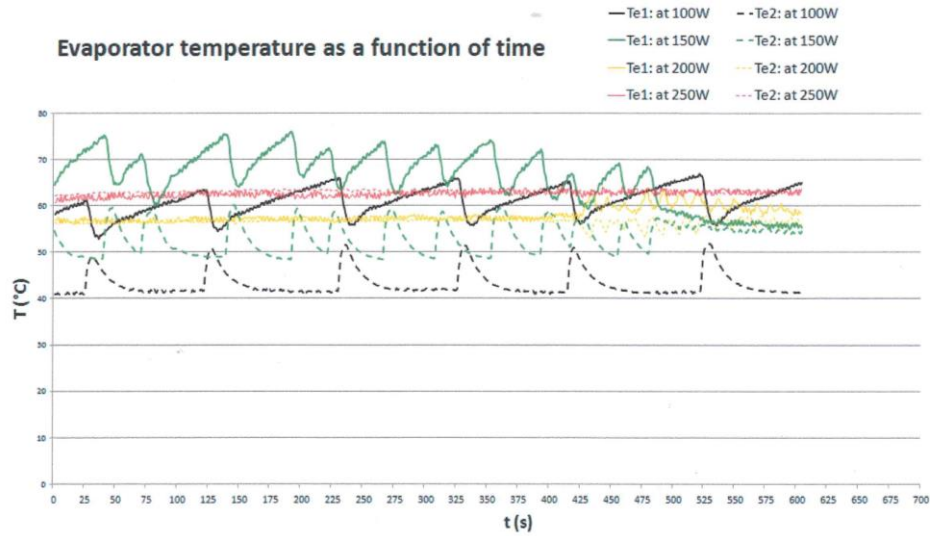
Figure 5. Evaporator temperatures for water-filled thermosyphon at different power throughputs
