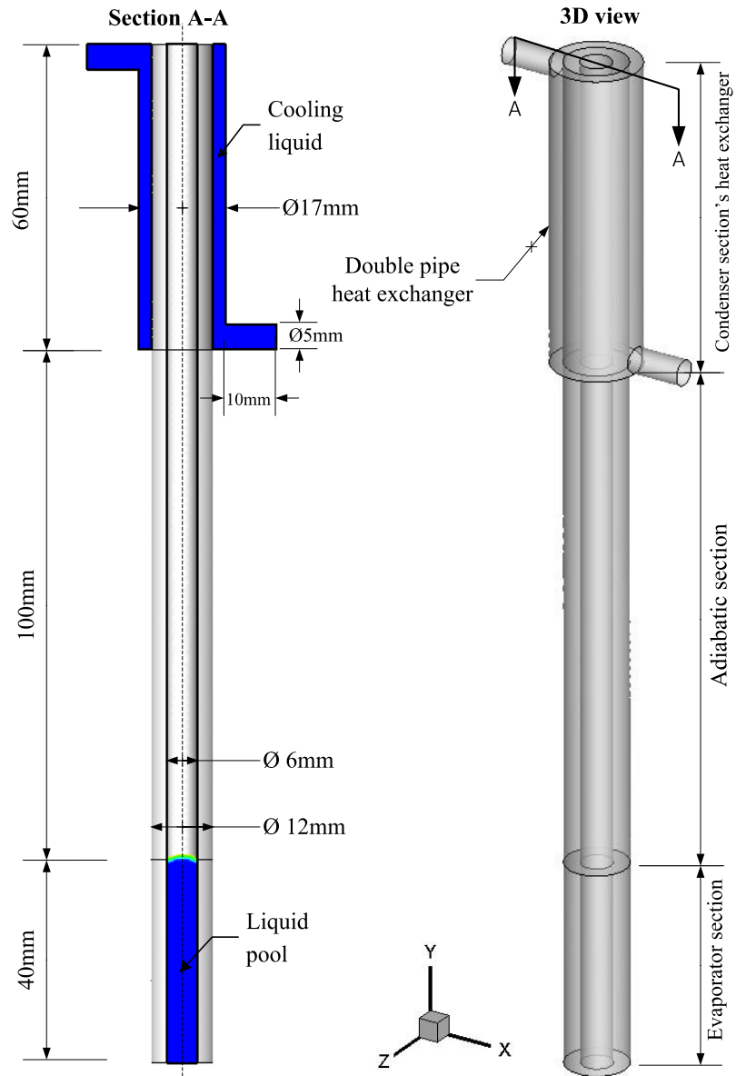
Figure 1: 3D model geometry and dimensions of two-phase closed thermosyphon with water jacket
