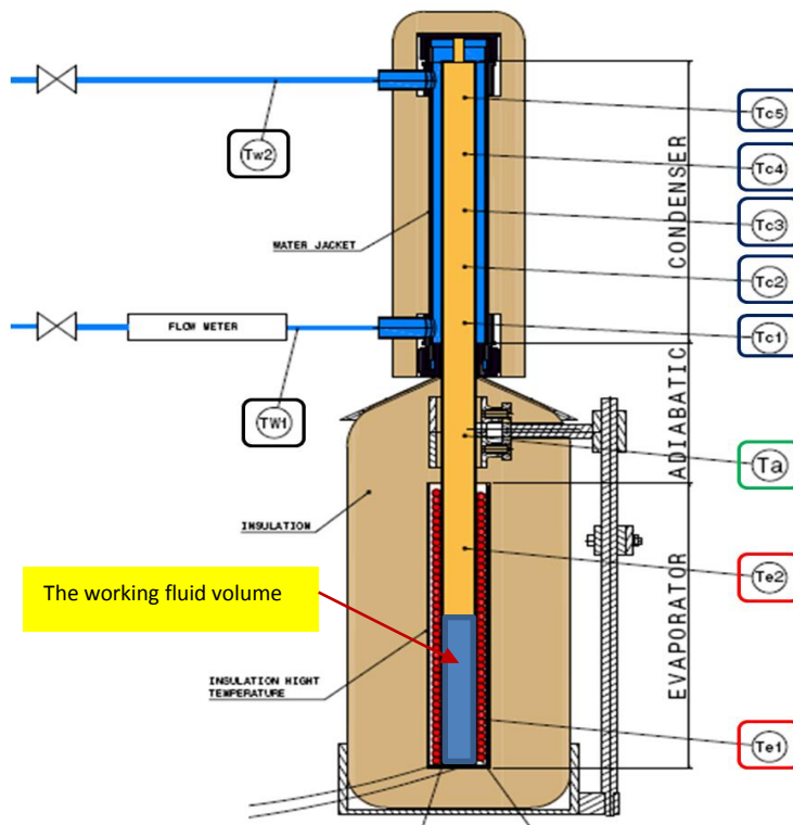
Figure 3. The experimental apparatus
