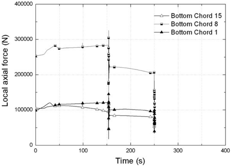
Figure 12. Bottom Chord axial forces for the 7th floor.
