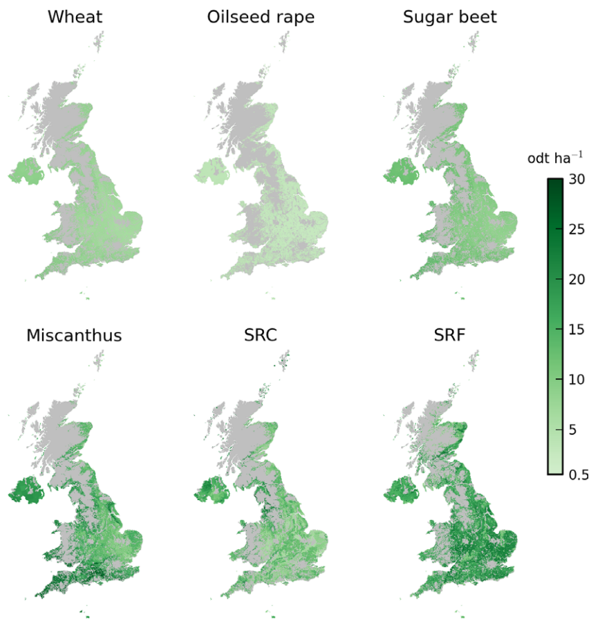
Fig. 2 Spatial distribution of modelled mean annual yield of bioenergy crops as odt ha -1 yr -1 (where odt is oven dry tonnes) in the 2030s under the UKCP09 medium emissions climate scenario. Miscanthus , SRC and SRF yields were obtained from simulations using the models MiscanFor, ForestGrowth SRC and ESC-CARBINE, respectively. Defra yield statistics from 2000 to 2008 were used to establish baseline yield values for wheat, OSR and sugar beet, which were then adjusted for future climate using the Miami model (see text).
