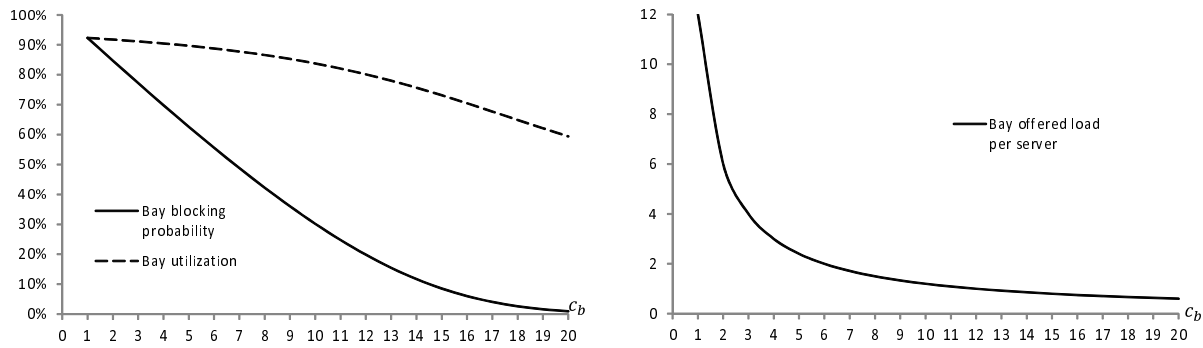
(a) Bay blocking probability ( \pi_1^b ) and bay utilization ( U_b ) (b) Bay offered load per server ( \rho_b )
