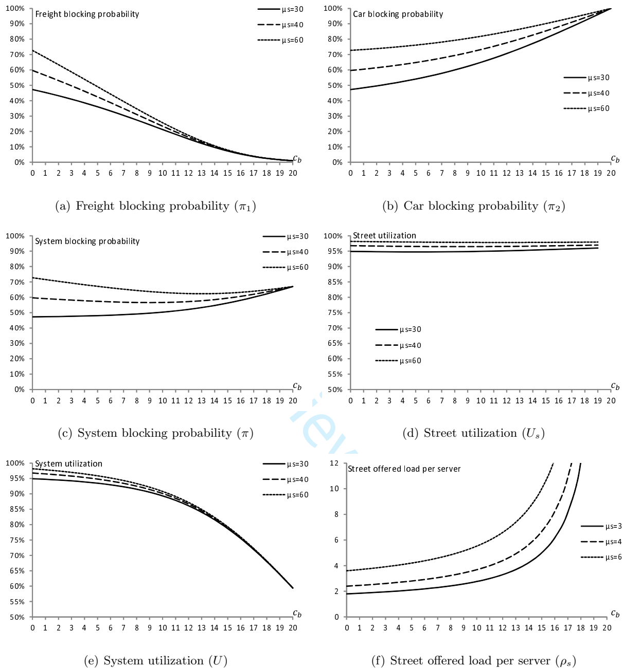
Figure 4 Street and system performance measures for Example 2 ( c = 20, \lambda_1 = 0.4, \lambda_2 = 0.8, \mu_b = 1/30, \mu_s = 1/30, 1/40, 1/60 )
