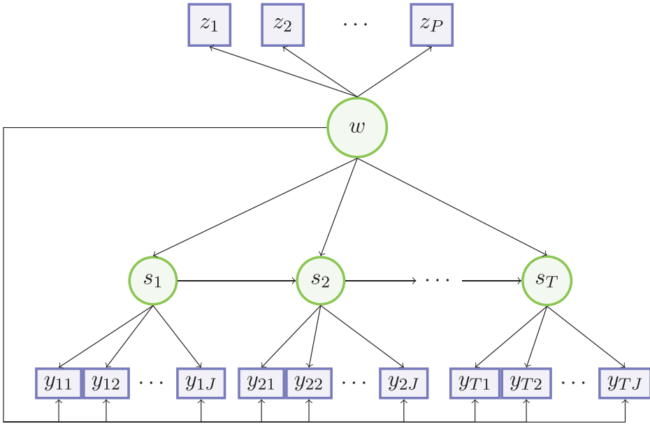
Figure 1. Graphical representation of MLM model. w : time-constant latent class variable; z : time-constant variables; s : dynamic latent variable; y : time-varying variables.
