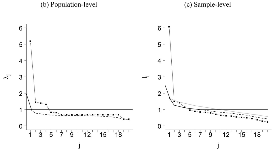
Figure 3. Example illustrating the Empirical Kaiser Criterion (EKC) with and without the greater-than-1 restriction. Note. Successive columns of (a) present the population eigenvalues ( \lambda_j ), population reference eigenvalues using the unrestricted EKC ( \lambda_j^{REF} ), sample eigenvalues ( l_j ), and its reference eigenvalues using parallel analysis ( l_j^{Parallel} ) and the unrestricted EKC ( l_j^{REF} ). The bold reference eigenvalues shows that EKC selects four factors in the example, whereas parallel analysis selects one factor. Panels (b) and (c) depict the same information for the population and sample respectively, with eigenvalues (black squares) and reference eigenvalues (black [dashed] solid line for [unrestricted] EKC and gray solid line for parallel analysis). EKC is identical to Kaiser’s greater-than-one rule at the population-level in panel (b).
