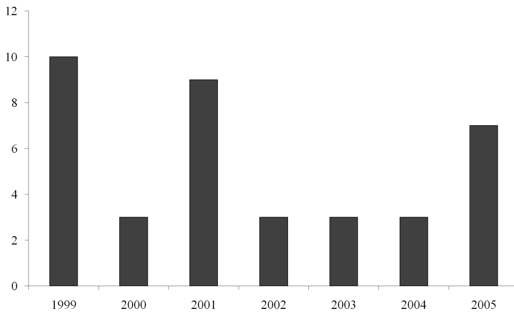
Figure 2.A.2: Distribution of first CDS engagements
