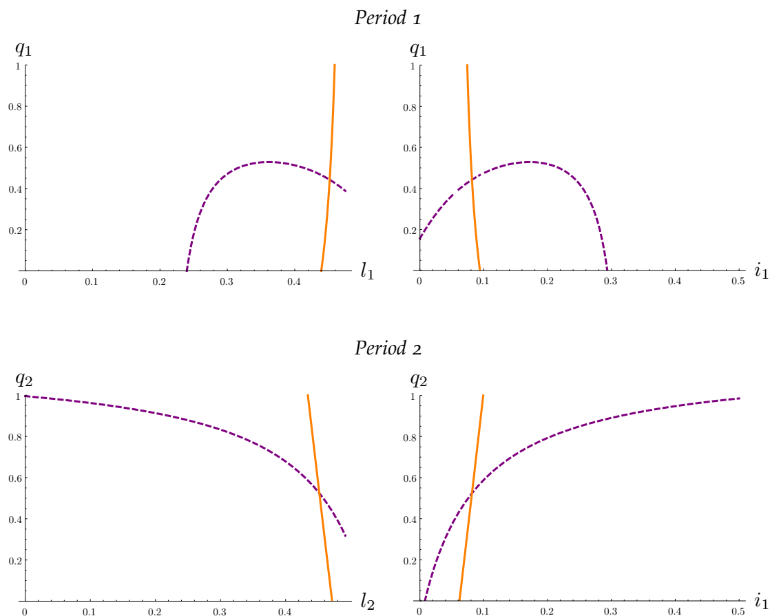
Figure 4.3: Reaction functions of the bank and the CBFS
