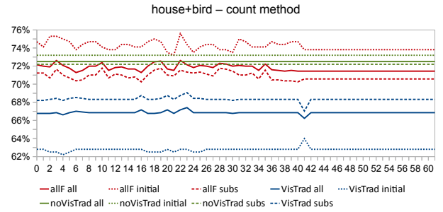
Figure 4: Accuracy for different visual contexts (determined by the count method) for the bird+house maps.
