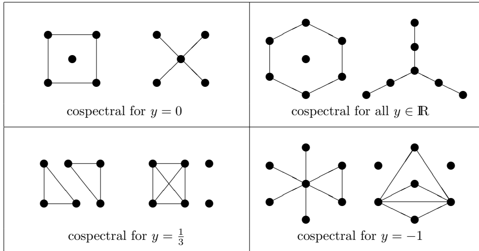
Figure 7: Examples of pairs of graphs with cospectral matrices A_G - yJ
