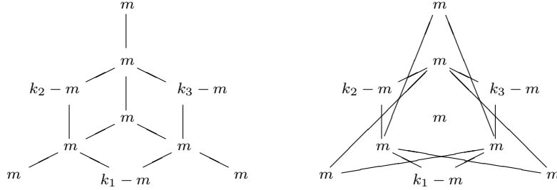
Figure 6: Quotients of switching equivalent graphs G_2 and H_2
