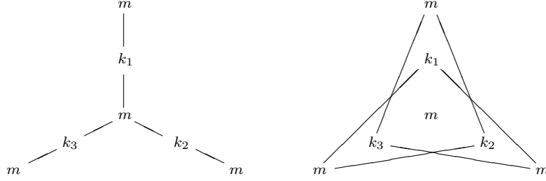
Figure 5: Quotients of switching equivalent graphs G_1 and H_1
