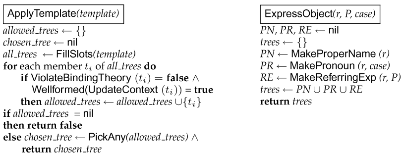
Figure 2 Functions ApplyTemplate (left) and ExpressObject (right).
