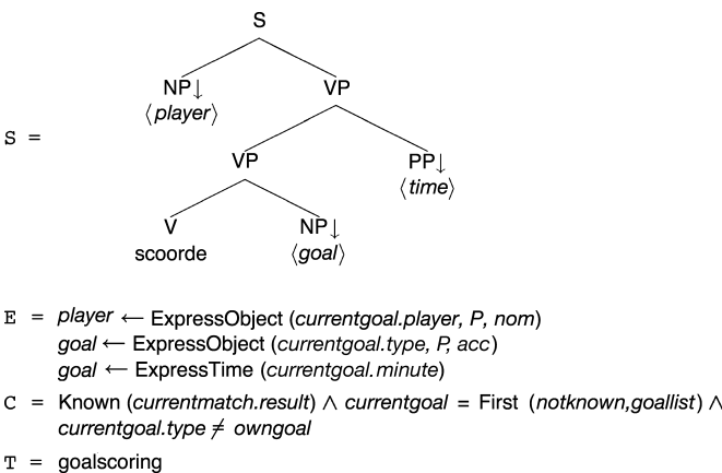
Figure 1 Sample syntactic template from the GOALGETTER system.
