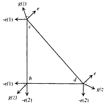
Fig. 3. Stationary points of g on \partial(\bar{r}) \cap \mathbb{R}^2_+ .
