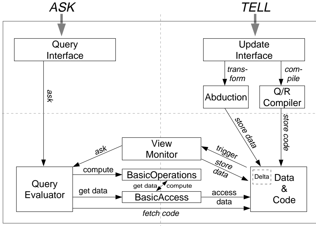
Figure 2: The Architecture of the ConceptBase Server
