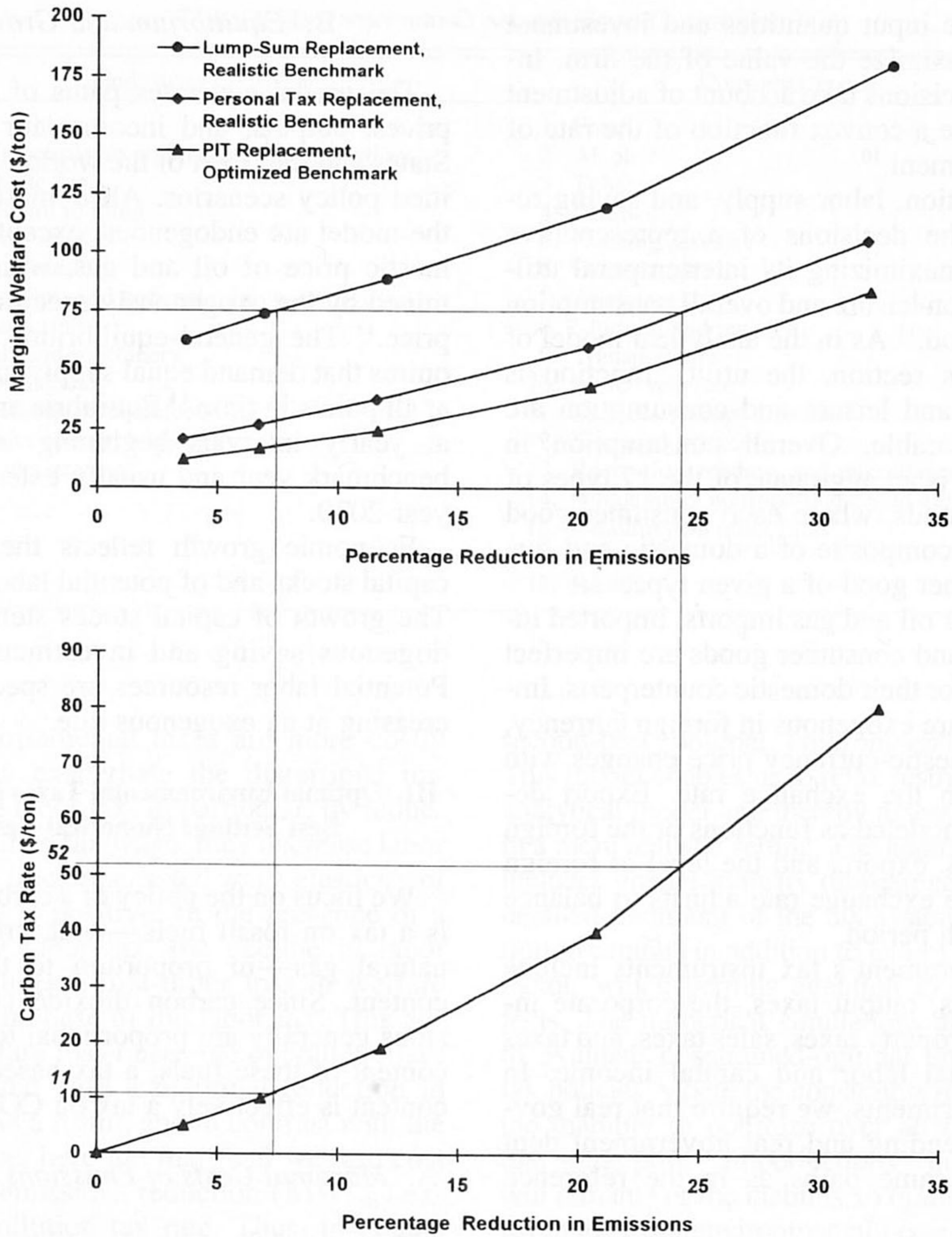
FIGURE 1. MARGINAL WELFARE COSTS, EMISSIONS REDUCTIONS, AND CARBON TAX RATES Note: 1A (upper graph) shows the marginal welfare costs of emission reductions. 1B (lower graph) shows the carbon taxes required for particular emissions reductions.
