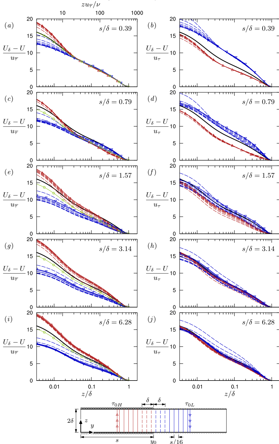
FIGURE 4. Local defect U_{\delta} - U \equiv U(y, \delta) - U(y, z) at various lateral ( y ) stations: scaled with the averaged friction velocity u_{\tau} , left panels, i.e. (a, c, e, g, i); scaled with the local friction velocity u_{\tau} = u_{\tau H} or u_{\tau L} , right panels, i.e. (b, d, f, h, j). Top to bottom, s/\delta \approx 0.39, 0.79, 1.57, 3.14, 6.28 ; —, uniform shear stress; \triangle , centre of high shear stress region; \nabla , centre of low shear stress region; \circ , global defect; \square , y in high shear stress region, dashed if within \delta of stress jump; \square , y in low shear stress region, dashed if within \delta of stress jump. See key at bottom.
