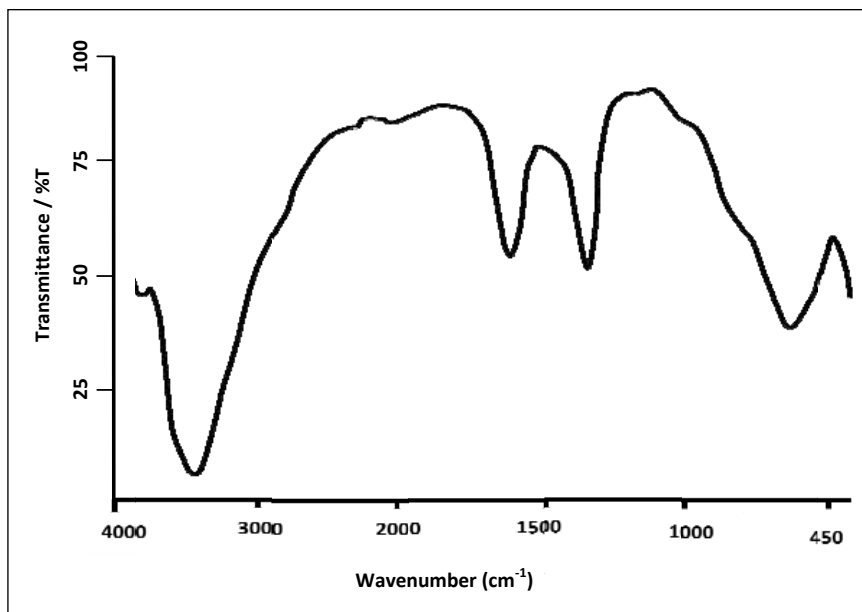
Figure 2: FTIR spectra for the synthesized MgAlCO_3 -LDH
