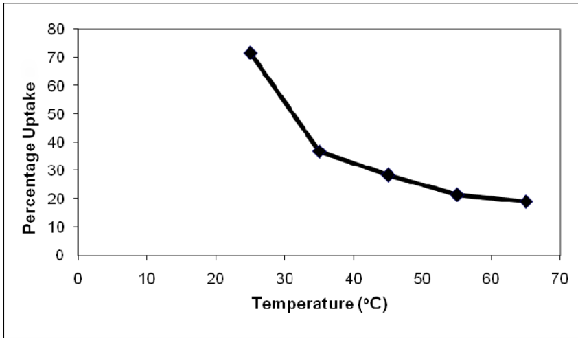
Figure 8: Cd(II) percentage uptake with temperature
