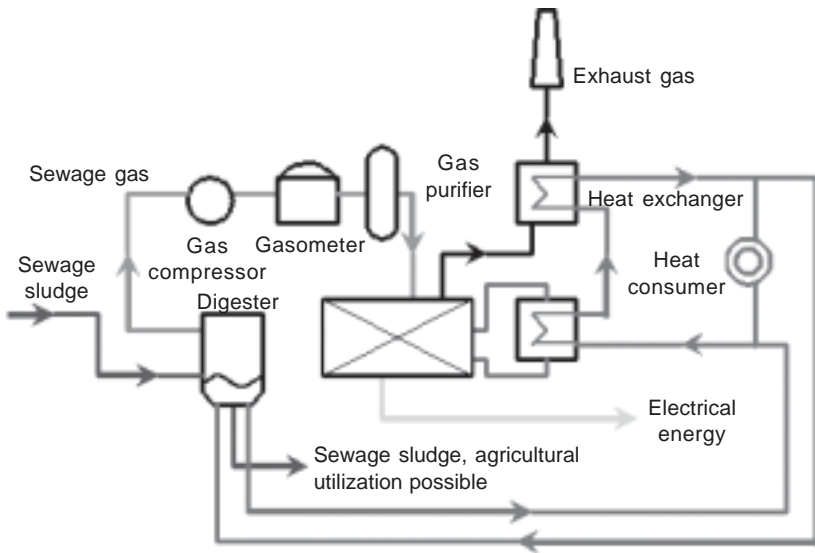
Figure 2: The Field Transformation of Sewage Sludge into Biogas, which in Turn Generates Electrical Energy [7]
