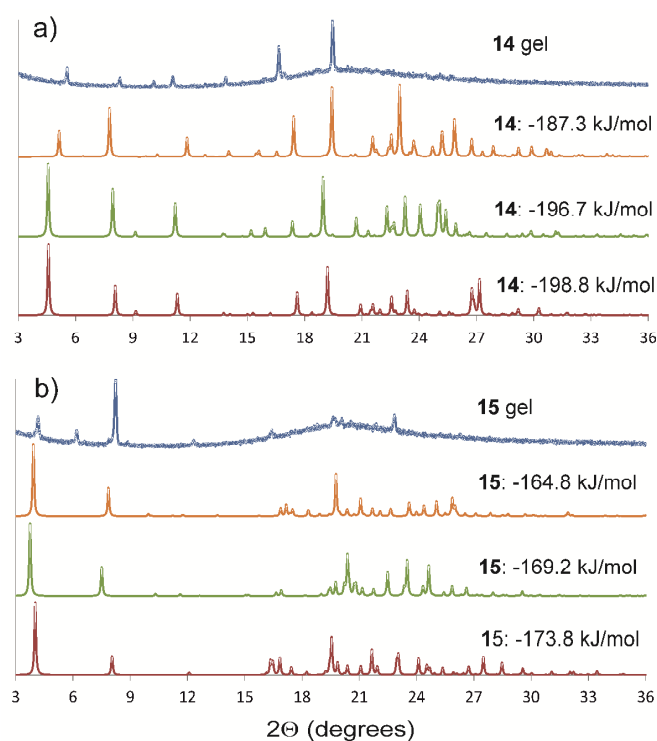
Fig. 5. Powder X-ray diffraction patterns of the gels (a) 14 and (b) 15 in DMSO, compared to simulated diffraction patterns from low energy predicted structures that give similar diffraction patterns to the gels. The simulated patterns from the predicted structures are labelled by their calculated lattice energies. The simulated diffraction patterns of 14 and 15 with lattice energies of -198.8 and -173.8 \text{ kJ mol}^{-1} correspond to the predicted crystal structures reported in Fig. 4a, 4e, respectively. A larger set of comparisons is provided in the supporting information. †
