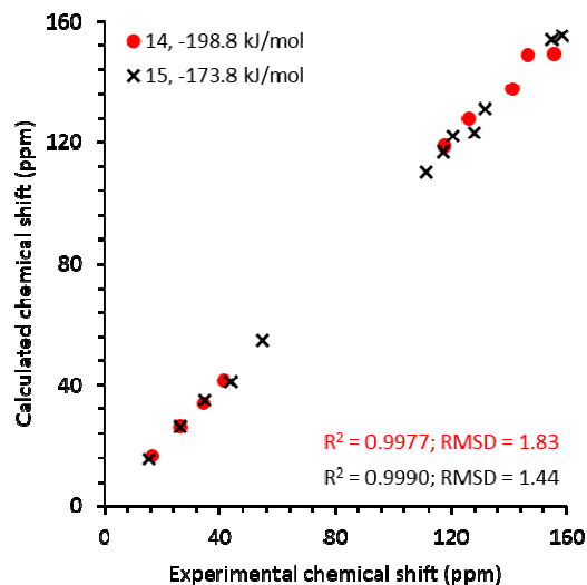
Fig. 9 Experimental 13 C chemical shift values for frozen gels 14 and 15 acquired at 0 °C and MAS rate of 8 kHz vs. calculated values for the predicted structures that give best agreement with both NMR and PXRD from the gel. Calculated isotropic chemical shieldings were converted to chemical shifts by matching the calculated and observed chemical shift of the CH 3 carbon in gel. The structures for gelators 14 and 15 correspond to those reported in Fig. 4a, 4e, respectively.
