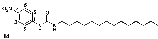
Fig. 8 Aromatic carbon labels for gelator 14 .
