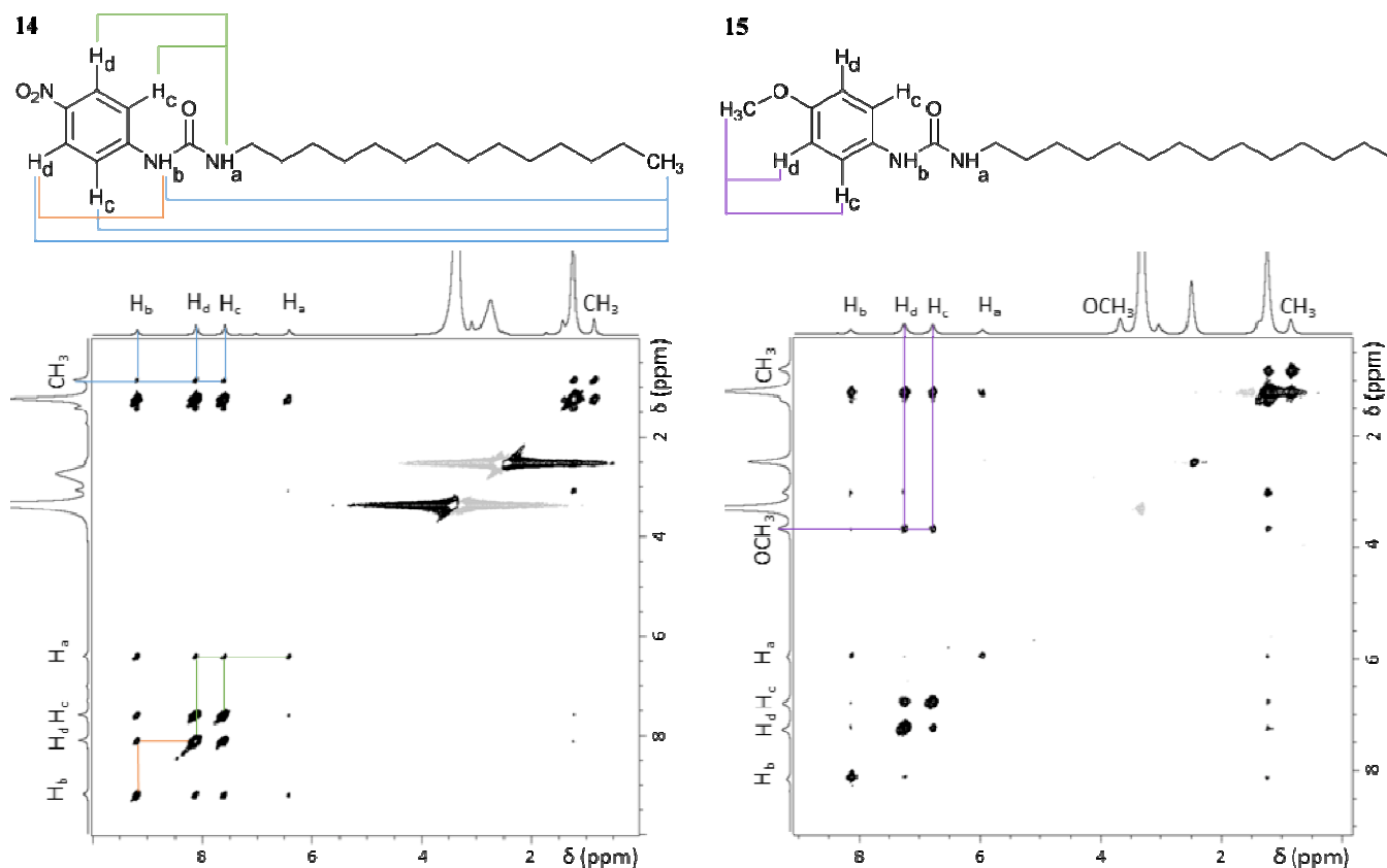
Fig. 6 2D ^1H - ^1H NOESY spectra of gels 14 and 15 ( 60\text{ mg mL}^{-1} in DMSO-d_6 ) were acquired at 25\text{ }^\circ\text{C} with a mixing time of 0.5\text{ s} using a 800.23\text{ MHz} spectrometer. Relevant cross-peaks have the corresponding spatial connectivity assigned (coloured lines). The cross-peaks observed between the -CH_2 and the aromatic protons in gel 15 do not contain structural information, as they result from indirect NOE enhancements, only observable at long mixing times † .
