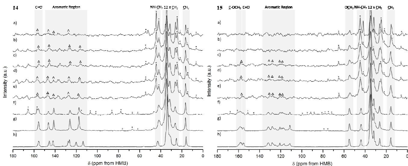
Fig. 7 ^1H - ^{13}C CP/MAS NMR spectra of gel samples ( 60\text{ mg mL}^{-1} in DMSO-d_6 ) acquired at 25\text{ }^\circ\text{C} and 1\text{ kHz} MAS rate (a), frozen gel samples acquired at 15\text{ }^\circ\text{C} (b), 10\text{ }^\circ\text{C} (c) and 5\text{ }^\circ\text{C} (d) and 1\text{ kHz} MAS rate, frozen gel samples acquired at 0\text{ }^\circ\text{C} and 1\text{ kHz} (e), 4\text{ kHz} (f) and 8\text{ kHz} (g) MAS rates, and reference solid powders acquired at 25\text{ }^\circ\text{C} and 10\text{ kHz} MAS rate (h) for 14 and 15 . Low-resolution aromatic peaks are highlighted with triangles ( \Delta ) and spinning sidebands with asterisks (*).
