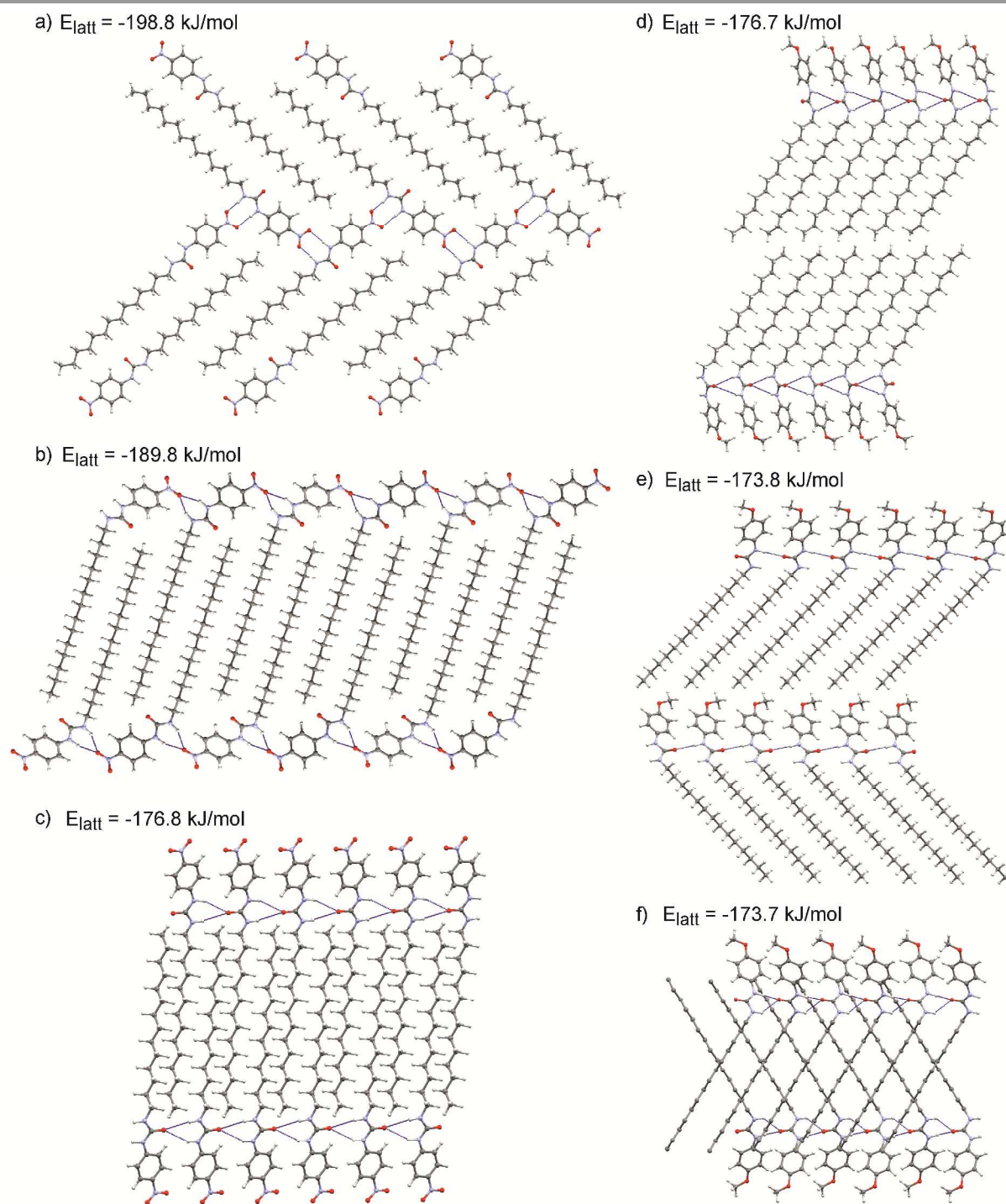
Fig. 4 Molecular packing in representative low energy predicted crystal structures of 14 (a, b, c) and 15 (d, e, f). a) and d) are the global minimum energy crystal structures that have been located for each molecule. Calculated lattice energies of each structure are shown. Hydrogen bonds are shown as dashed blue lines. hydrogen atoms on the alkyl chains are hidden in (f) for clarity.
