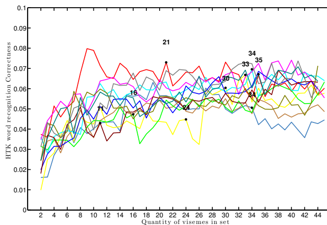
Fig. 1: Viseme correctness as the quantity of visemes changes in a set of classifiers for 12 LiLiR speakers. Results from [13].
