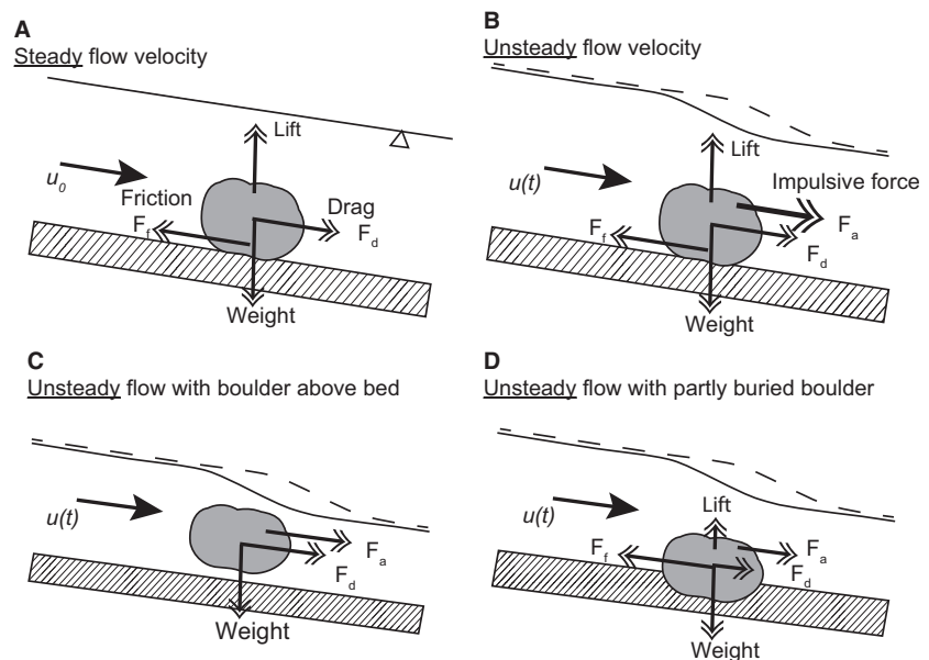
Fig. 3. Simple sketches of forces acting on a boulder in different settings. The top lines in each drawing represent the instantaneous position of the moving water surface. (A) Forces of drag F_d and friction F_f on a boulder in steady water flow. (B) The forces on the same boulder in a flow that has a rapidly changing velocity, including the impulsive force F_a . (C) Sketch of the position of a boulder above the bed with neither friction nor lift. (D) Forces on a partly buried boulder.
