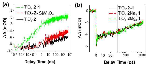
Fig. 5 (a) Ground state bleach recovery kinetics of TiO 2 -2 (black), TiO 2 -2-SiW 12 O 40 (red) and TiO 2 -2-1. (b) Ground state bleach recovery kinetics of TiO 2 -2-1 (black), TiO 2 -2-Na 2 -1 (red) and TiO 2 -2-Mg 2 -1 (green).
