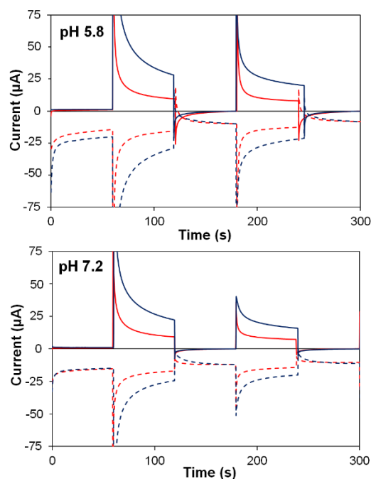
Fig. 8 Photoelectrochemical generator-collector measurements (chronoamperometry) of TiO 2 - P2-1 (red) and TiO 2 - 2Na 2 -1 (dark blue) at pH 5.8 and pH 7.2. Solid lines, photoanode current; dashed lines, collector current; collector efficiency ca. 60%. Applied bias 0 mV vs Ag/AgCl, illuminated with a 455 nm LED (33 mW cm -2 ). Photocurrent densities are reported in Table 5.
