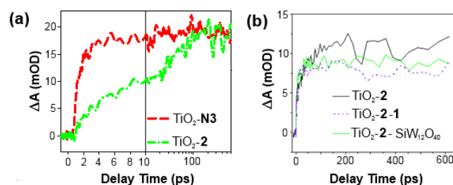
Fig. 4 Mid-IR comparison of the kinetics of electron injection in (a) TiO 2 - 2 and TiO 2 - N3 , and; (b) TiO 2 - 2-1 and TiO 2 - 2-SiW 12 O 40 . Data have been scaled to the absorbance of the supporting dyad film.
