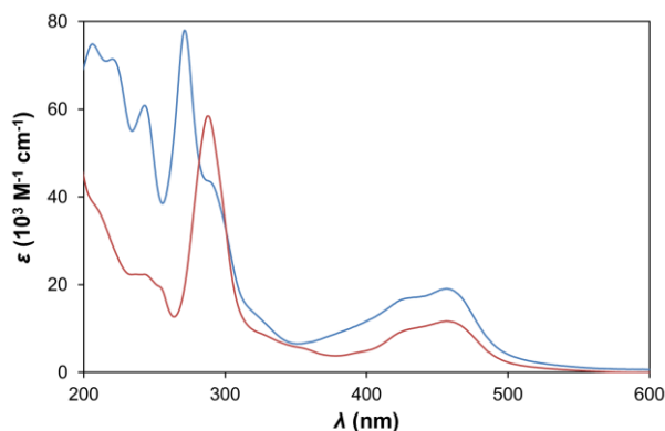
Fig. 3 UV-vis spectra of H 2 2 (blue) and P 2 (red) in H 2 O at 298 K.
