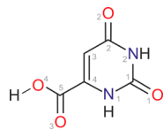
Figure 1. Molecular diagram of orotic acid (uracil-4-carboxylic acid, OTA).
