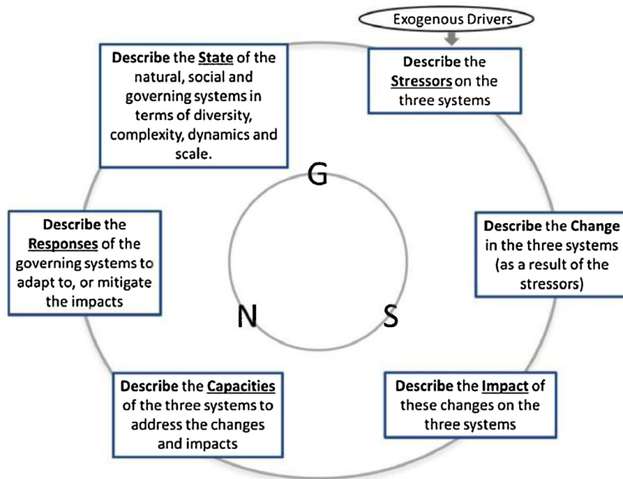
Fig. 7. The Description and response component of I(IMBER)-ADApT, which includes the Natural (N), Social (S) and Governing Systems (G). The outer circle represents a continuous cycle, which can be entered at any point, and the inner circle indicates that each component of the Description should be applied to the natural, social and governing systems. From Bundy et al. (2015).
