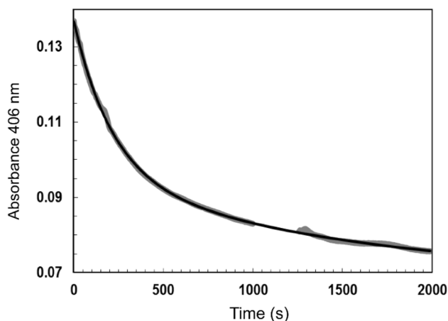
Fig. 5 Kinetics of O 2 -mediated [4Fe-4S] cluster conversion. Kinetics were recorded under pseudo-first-order conditions (8.5 \mu M [4Fe-4S], 161.6 \mu M O 2 ) at an [O 2 ]:[4Fe-4S] ratio of 19 at 25 °C. A double exponential function (black line) was used to fit the data (gray). The rate constants reported in the text from these experiments are mean values with standard errors from two repeats
