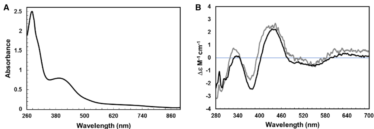
Fig. 2 Spectroscopic properties of [4Fe-4S] FnrP. a. Absorbance spectrum of reconstituted FnrP (48 \mu M [4Fe-4S], 81 % cluster loaded), b CD spectrum of the same reconstituted FnrP (black) and
