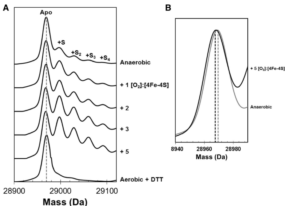
Fig. 4 Detection of persulfide species of FnrP by LC-MS.
