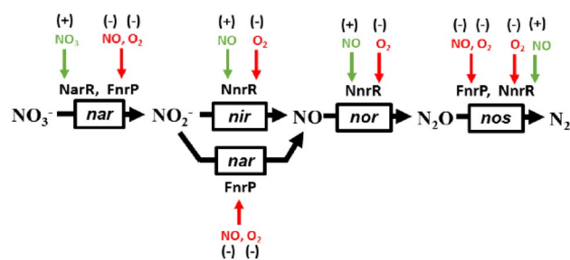
Fig. 1 Regulation of denitrification in P. denitrificans . Nitrate reductase ( nar ) is co-regulated by NarR and FnrP. Nitrite reductase ( nir ) and nitric oxide reductase ( nor ) are regulated solely by NnrR. Nitrous oxide reductase ( nos ) is co-regulated by FnrP and NnrR. Summarized from references [4, 10, 11, 14]. Small molecule effectors required to activate or inhibit transcription are marked a (+) or (-), respectively. Note: under certain circumstances nar will reduce nitrite (NO 2 - ) to nitric oxide (NO)
