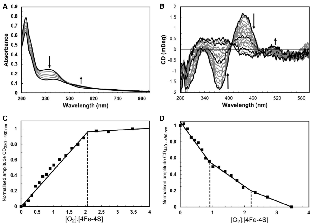
Fig. 3 Titration of [4Fe-4S] FnrP with oxygen. a Absorbance spectra following addition of O_2 to [4Fe-4S] FnrP (15 \mu M in cluster). Black lines represent an [O_2]:[4Fe-4S] ratio of 0 and 5, respectively. b CD spectra following addition of O_2 to [4Fe-4S] FnrP (16 \mu M in cluster) monitored by circular dichroism. Black lines represent [O_2]:[4Fe-
