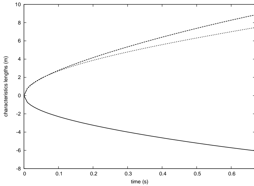
Figure 4: Time variations of positions of 3 points of the contact line: front point x_p (dashed line), rear point x_m (solid line) and lateral point y_p (dotted line).
