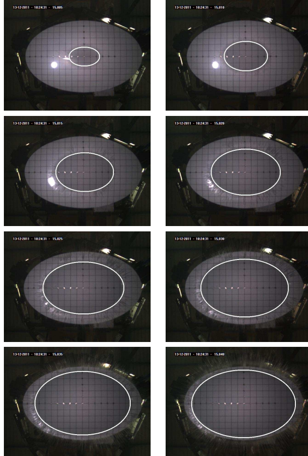
Figure 2: Snapshots of the expanding wetted surface for an oblique entry of elliptic paraboloid defined by R_x = 0.75m , R_y = 2m . The experimental set-up is described in [Scolan(2012)]. The constant vertical velocity and y -horizontal velocity are \dot{h} = 0.79m/s and \dot{y}_b = 0.59m/s respectively. There are no rotations in the experiments. The camera records at 200Hz. The periphery of the wetted area of the body surface at different time instants is marked by a thick white line.
