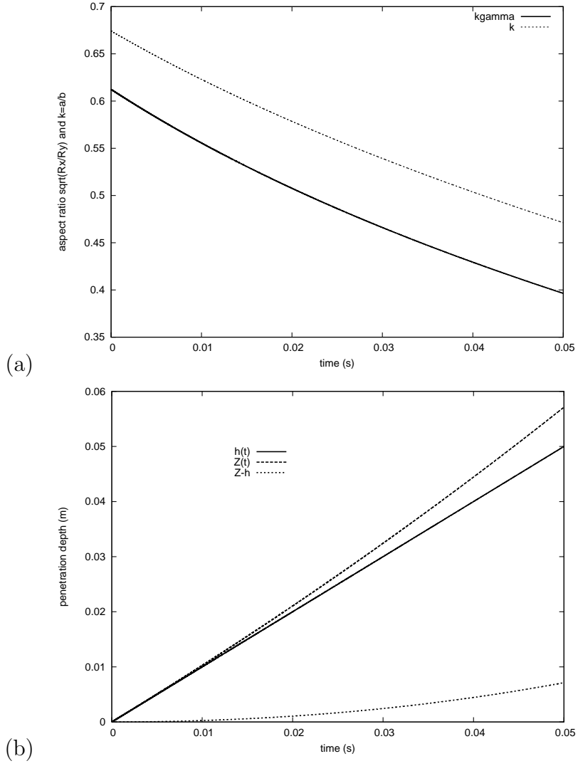
Figure 6: Time variation of (a) the aspect ratios k_{\gamma} = \sqrt{R_x/R_y} (solid line) and k = a/b (dashed line), (b) the penetration depth h (solid line), the modified penetration depth Z (dashed line) and the difference Z - h (dotted line) .
