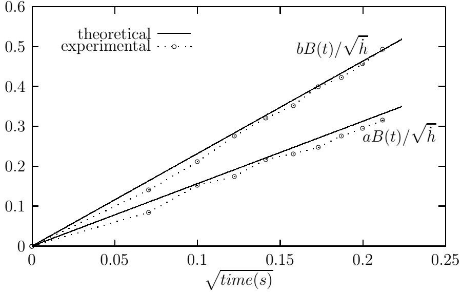
Figure 3: Time variations of the major and minor semi-axes of the elliptic wetted surface, respectively bB(t) and aB(t) , divided by \sqrt{h} . Comparison of experimental data (marks) and theoretical results (solid lines). The vertical velocity and y -horizontal velocity are \dot{h} = 0.79m/s and \dot{y}_b = 0.59m/s respectively.
