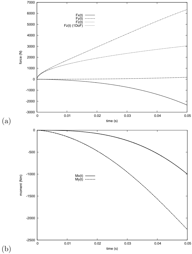
Figure 9: Time variation of (a) horizontal and vertical forces for 7 DoF and 1 DoF, (b) moment around the two horizontal axes. For 7 DoF, the time variations of parameters (h, R_x, R_y, \alpha_x, \alpha_y, x_b, y_b) are the same as in figure (6).
