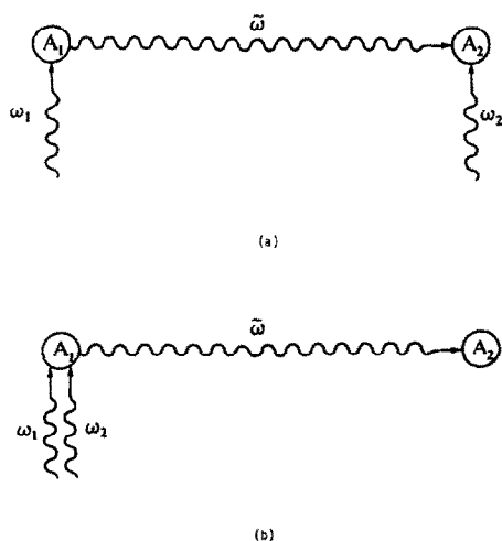
Fig. 3. Two mechanisms for synergistic absorption of photons, \omega_1 , \omega_2 ; (a) shows the cooperative mechanism and (b) the distributive mechanism. In each case the energy mismatch is mediated by a virtual photon \bar{\omega} .
