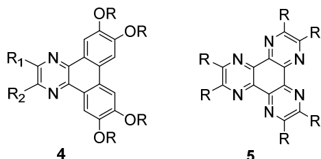
Figure 2. Electron deficient azatriphenylenes.
