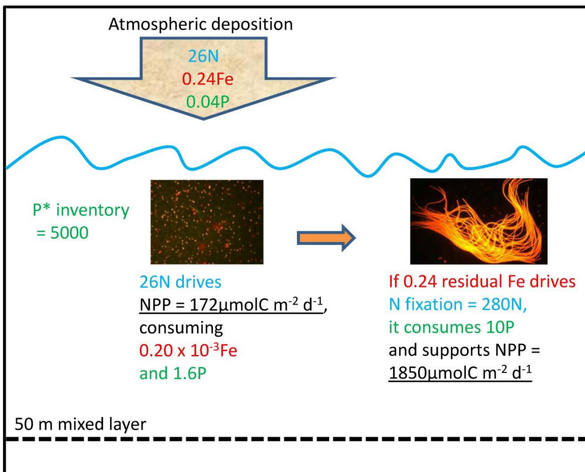
Figure 5 Summary of calculated impacts of atmospheric deposition of nitrogen (blue), iron (red) phosphorus (green) on water column net primary production (NPP) (all rates are as \mu\text{mol m}^{-2} \text{d}^{-1} ) with a water column P^* of 0.1 \mu\text{mol l}^{-1} , and hence P^* inventory ( P^* ) as \mu\text{mol m}^{-2} for a 50 m surface mixed layer. See text for details.
