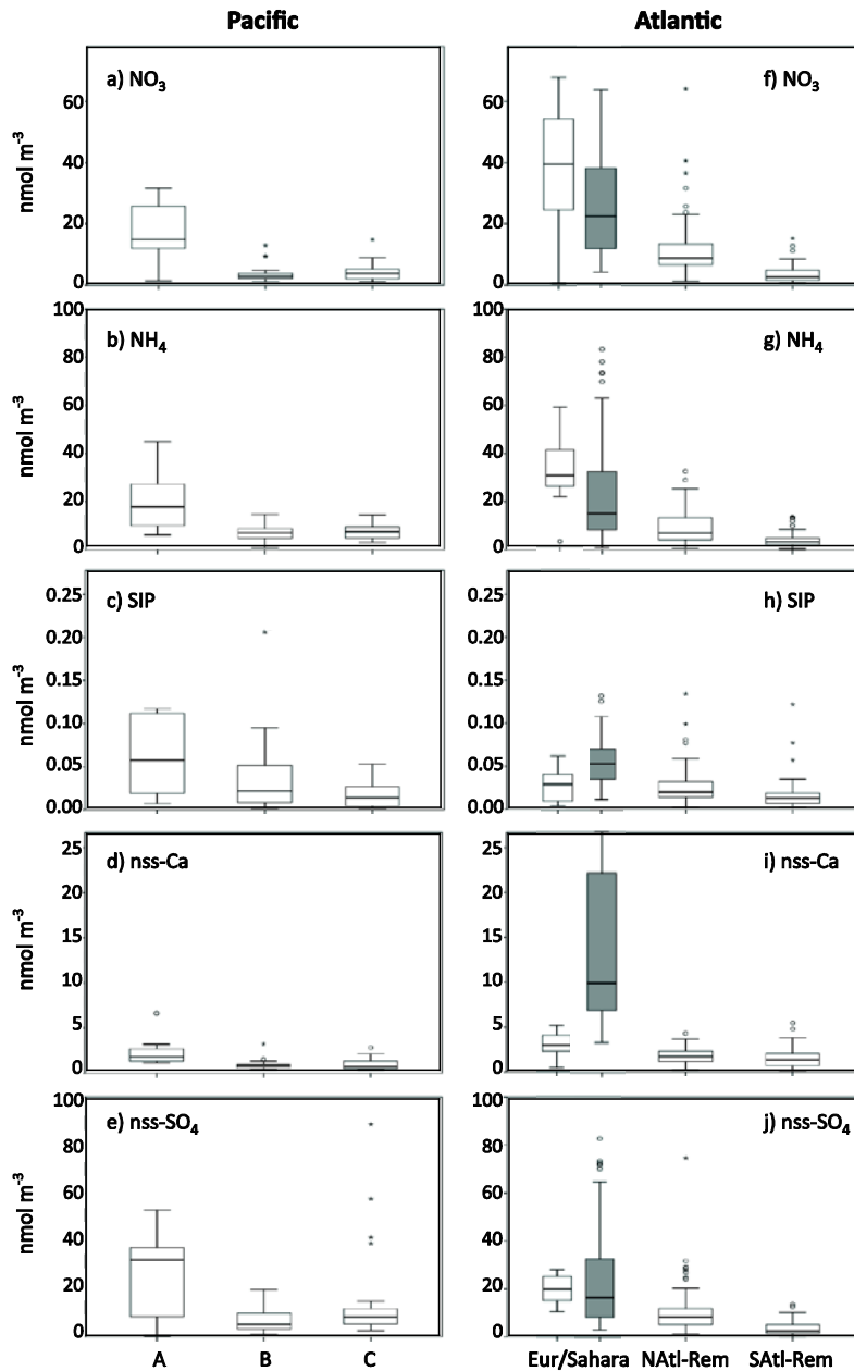
Fig 4 Box and whisker plots showing the distribution of nitrate, ammonium, SIP, nssCa and non-sea-salt sulphate (panels a – e) for zones A, B and C in the Pacific sampled here. Panels f – j show distributions of these species in equivalent air masses sampled in the Atlantic ocean (data from Baker et al. [2010]). Note that 2 negative points for \text{nss-Ca}^{2+} and \text{nss-SO}_4^{2-} are excluded from these plots. The Saharan flow regime data is highlighted to aid comparison to other regions.
