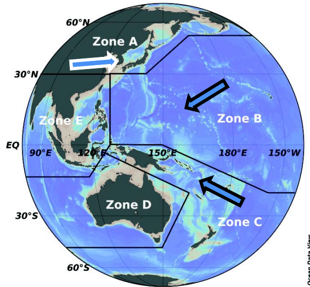
Figure 2: Classification of air mass back trajectory zones. Zone A: Asia. Zone B: Open Pacific. Zone C: Indonesia/Micronesia/New Zealand and Southern Ocean. Zone D: Australia. Zone E: Southern Asia. Main air flow regimes of relevance to this paper are indicated.
