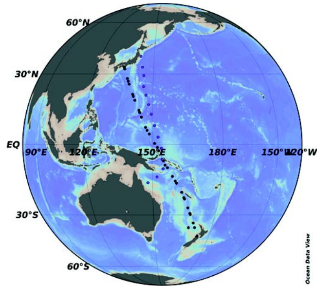
Figure 1: Sample start positions for the four Transfuture 5 (TF5) (black dots) and TransBrom (purple dots) cruises. Cruise dates were: TF5-1 May/June 2007; TF5-2 April/May 2008; TF5-3 August/September 2008; TF5-5 October/ November 2009; TransBrom October 2009.
