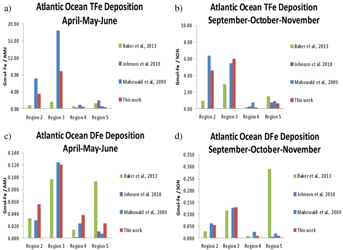
Figure 7. Comparison of Total Fe (TFe) and Dissolved Fe (DFe) input estimates to four Atlantic Ocean regions during the April-May-June (AMJ; left panels: a, c) and September-October-November (SON; right panels: b, d) periods (in Gmol-Fe) as compiled by Baker et al. (2013).
