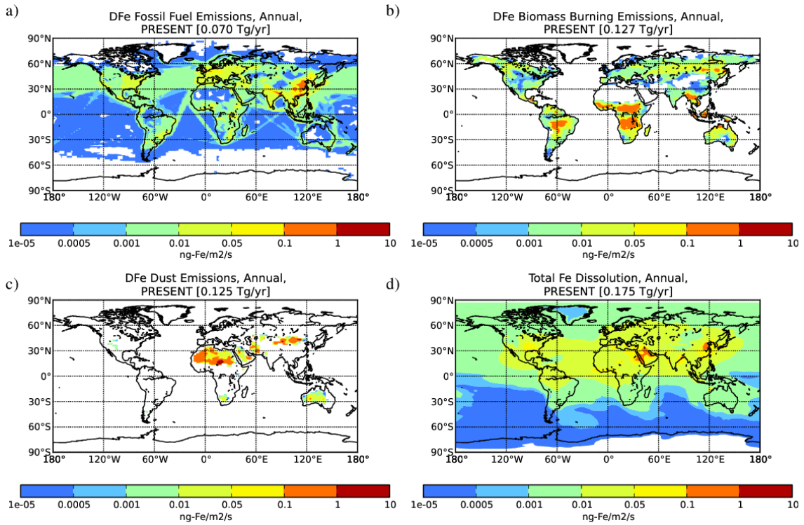
Figure 2. Annual averaged distributions (in \text{ng-Fe m}^{-2} \text{s}^{-1} ) of a) total anthropogenic DFe primary emissions, b) total biomass burning DFe emissions, c) total DFe mineral emissions and d) total mineral-Fe dissolution flux as calculated by TM4-ECPL for the present atmosphere.
