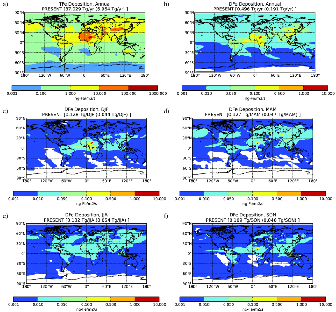
Figure 6. Calculated present annual deposition (in \text{ng-Fe m}^{-2} \text{ s}^{-1} ) for a) TFe, b) DFe, and the seasonal DFe deposition fluxes for c) December, January and February (DJF), d) March, April and May (MAM), e) June, July and August (JJA) and f) September, October and November (SON). In brackets (parentheses) the amounts of Fe deposition over the globe (only over oceans) are provided.
