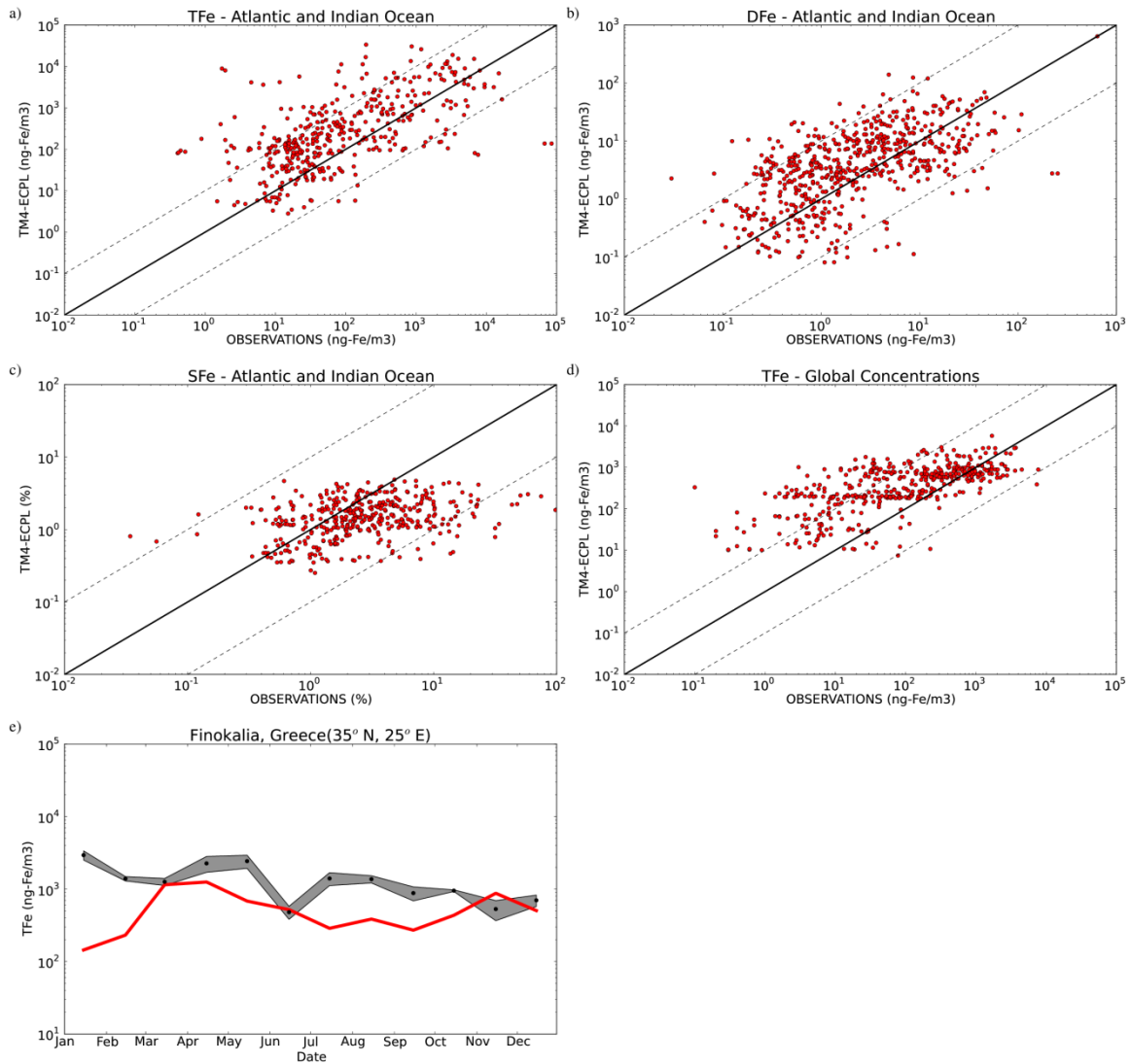
Figure 5. Log-scatter plot of model (y-axis) comparison with cruises observations over the Atlantic Ocean (Baker et al., 2013) and Indian Ocean (Witt et al., 2006) (x-axis) for a) TFe, b) the DFe and c) the SFe fractions in ambient aerosols, d) TFe comparison with global observations from Mahowland et al. (2005) and e) timeseries of monthly variation of TFe in ambient aerosols at Finokalia station (Koulouri et al., 2008); monthly mean observations are marked with dots, their variability is shown with the dashed area, model results are plotted by the black continuous line. In the scatter plots, the continuous black line shows the 1:1 correlation, while the dashed lines show the 10:1 and 1:10 relationships.
