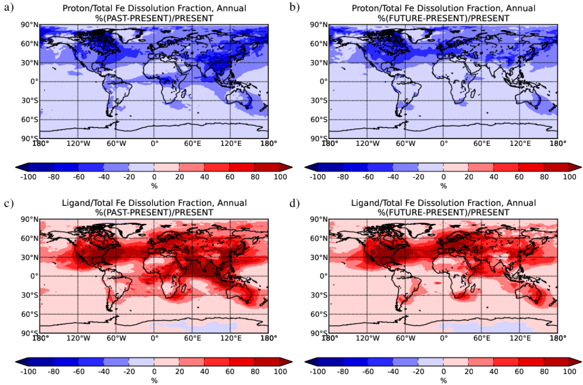
Figure 8. The percentage differences of PAST (left panels: a, c, e) and FUTURE (right panels: b, d, f) simulations from the PRESENT simulation for a, b) Proton-promoted/Total mineral-Fe Dissolution Fraction and c, d) Ligand-promoted/Total mineral-Fe Dissolution Fraction.
