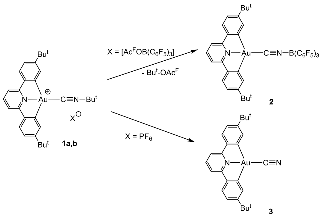
Scheme 2. Decomposition reactions of Au(III) isocyanide complexes.
