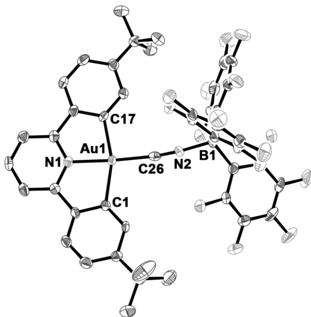
Figure 2. Structure of (\text{C}^{\wedge}\text{N}^{\wedge}\text{C})\text{Au-CN-B}(\text{C}_6\text{F}_5)_3 \cdot 0.5\text{CH}_2\text{Cl}_2 ( 2 \cdot 0.5\text{CH}_2\text{Cl}_2 ). Selected bond distances (Å) and angles (°): Au-C(26) 1.964(7), C(26)-N(2) 1.138(8), N(2)-B 1.593(9), N(1)-Au 1.988(5); Au-C(26)-N(2) 172.9(6). Thermal ellipsoids are set at 50% probability level. Hydrogen atoms and solvent molecules are omitted.
