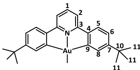
Figure 5. Numbering scheme of the C ^ N ^ C ligand.
