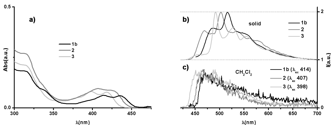
Figure 3. (a) Low energy region of the UV-Vis electronic spectra for complexes 1b , 2 and 3 in CH 2 Cl 2 solution. (b) Emission spectra of complexes 1b , 2 and 3 in the solid state at 298 K. (c) Emission spectra of complexes 1b , 2 and 3 in CH 2 Cl 2 solution under excitation at the lower energy absorption band.
