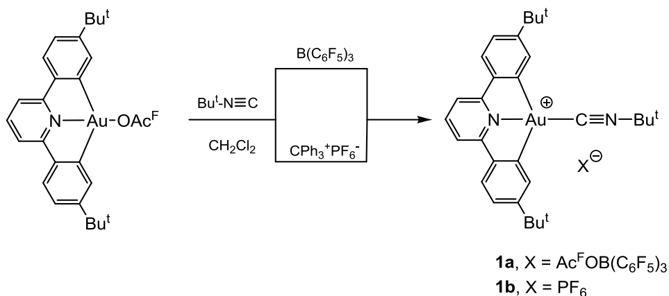
Scheme 1 Synthesis of (\text{C}^{\wedge}\text{N}^{\wedge}\text{C})\text{Au} isocyanide complexes
