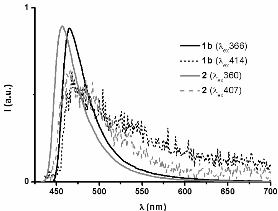
Figure 4. Emission spectra of complexes 1b and 2 in \text{CH}_2\text{Cl}_2 solution when excited by UV light of different energies
