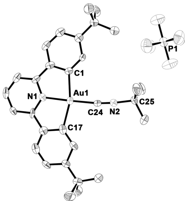
Figure 1. Structure of [(\text{C}^{\wedge}\text{N}^{\wedge}\text{C})\text{AuCN}^t\text{Bu}]\text{PF}_6 \cdot \text{CH}_2\text{Cl}_2 ( 1b · \text{CH}_2\text{Cl}_2 ). Selected bond distances ( \text{\AA} ) and angles ( ^\circ ): Au-C(24) 1.964(12), C(24)-N(2) 1.141(13), N(1)-Au 1.994(9); Au-C(24)-N(2) 173.4(10).
