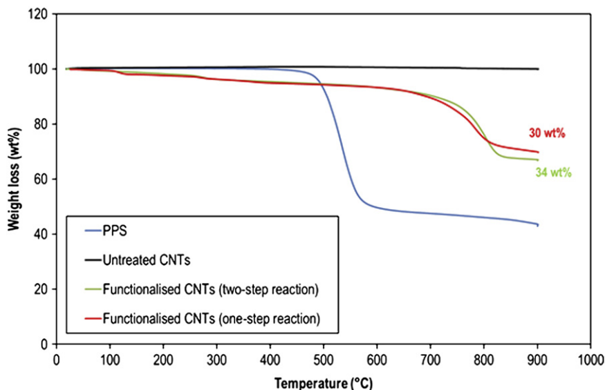
Fig. 9. TGA results of the pure PPS, untreated CNTs and functionalized CNTs in two-step and in a single step reaction.
