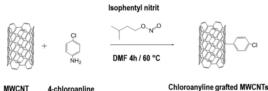
Fig. 3. Grafting of chloroaniline on the surface of the MWCNTs using a diazonium salt reaction.
