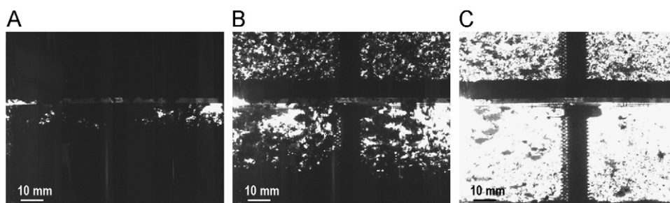
Fig. 5. FCNTs sedimentation after reaction. (A) 10 s after the oscillation stops. (B) 60 s after the oscillation stops. (C) 120 s after the oscillation stops.
