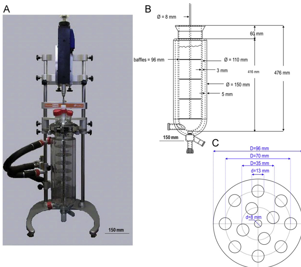
Fig. 1. 3 l oscillatory flow reactor (OFR). (A) Photograph of reaction vessel connected to the oscillation system. (B) Dimensions of the vessel. (C) Dimensions of the baffles.
