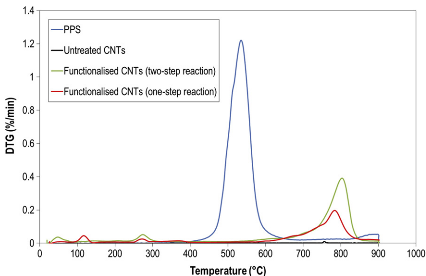
Fig. 10. DTG results of the pure PPS, untreated CNTs and functionalized CNTs in two-step and in a single step reaction.
