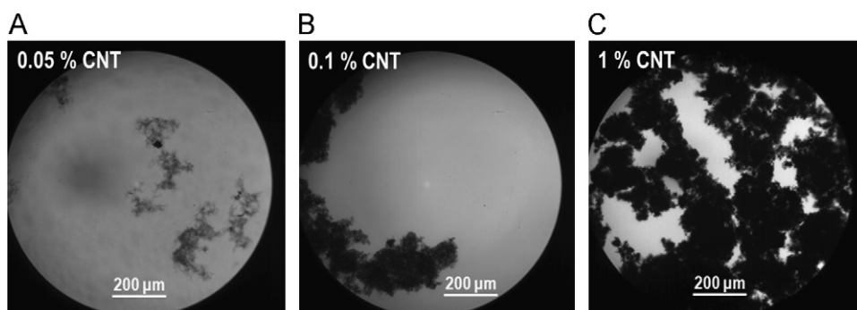
Fig. 6. Micrographs of CNT dispersions in DMF sonicated by means of a bioruptor for 1 h. (A), (B) and (C) corresponding to different sample concentrations 0.05 wt%, 0.1 wt% and 1 wt%.
