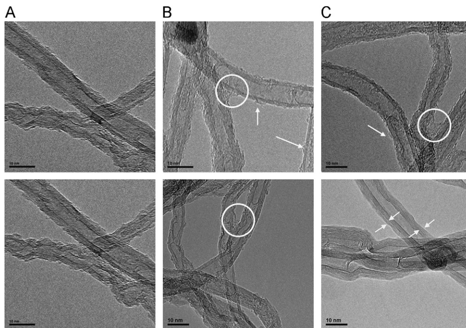
Fig. 7. TEM micrographs of CNTs (A) Untreated CNTs; (B) FCNTs from two stage OFR reaction (C) FCNTs from single stage OFR reaction.
