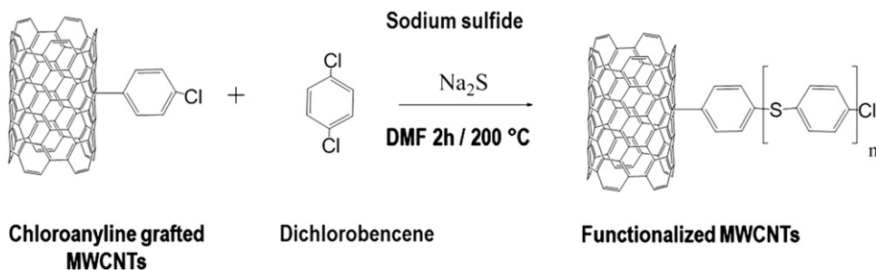
Fig. 4. Anchoring of PPS compatible chains on the surface of the modified MWCNTs.
