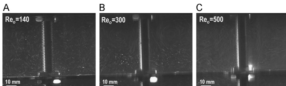
Fig. 2. Visualization of flow in the OFR. Tracer PS 125 \mu\text{m} . (A) Oscillatory conditions: frequency 1 Hz, amplitude centre to peak 5 mm (approx. Re_o = 140 ). (B) Oscillatory conditions: frequency 1 Hz, amplitude centre to peak 10.5 mm (approx. Re_o = 300 ). (C) Oscillatory conditions: frequency 2 Hz, amplitude centre to peak 8.5 mm (approx. Re_o = 500 ).
