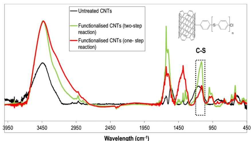
Fig. 8. FTIR spectra of the functionalized CNTs in two-step and in a single step reaction.
