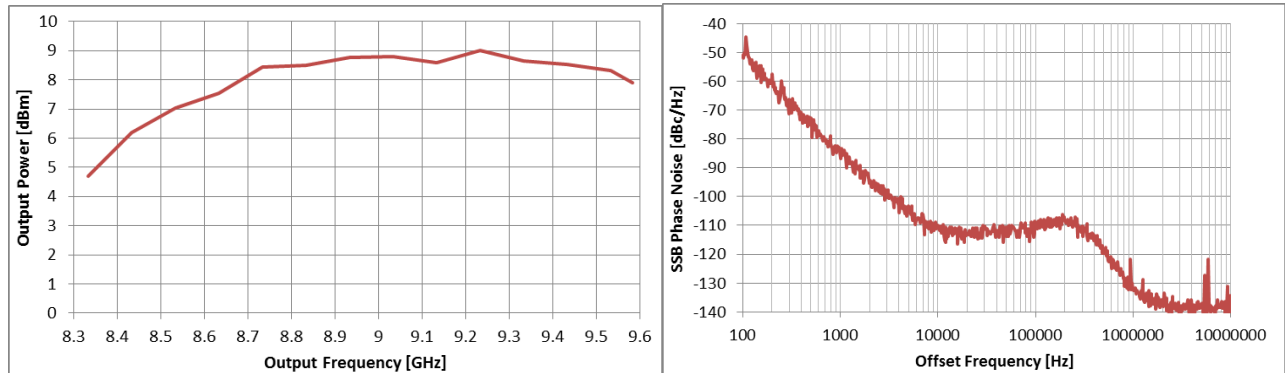
Figure 2. Chirp generator output power versus frequency (left) and CW phase noise at 8.953 GHz (right).
