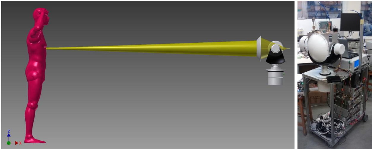
Figure 1. CAD model of Pathfinder 220 GHz radar scanning a mannequin (left). Photograph of Pathfinder radar (right).
