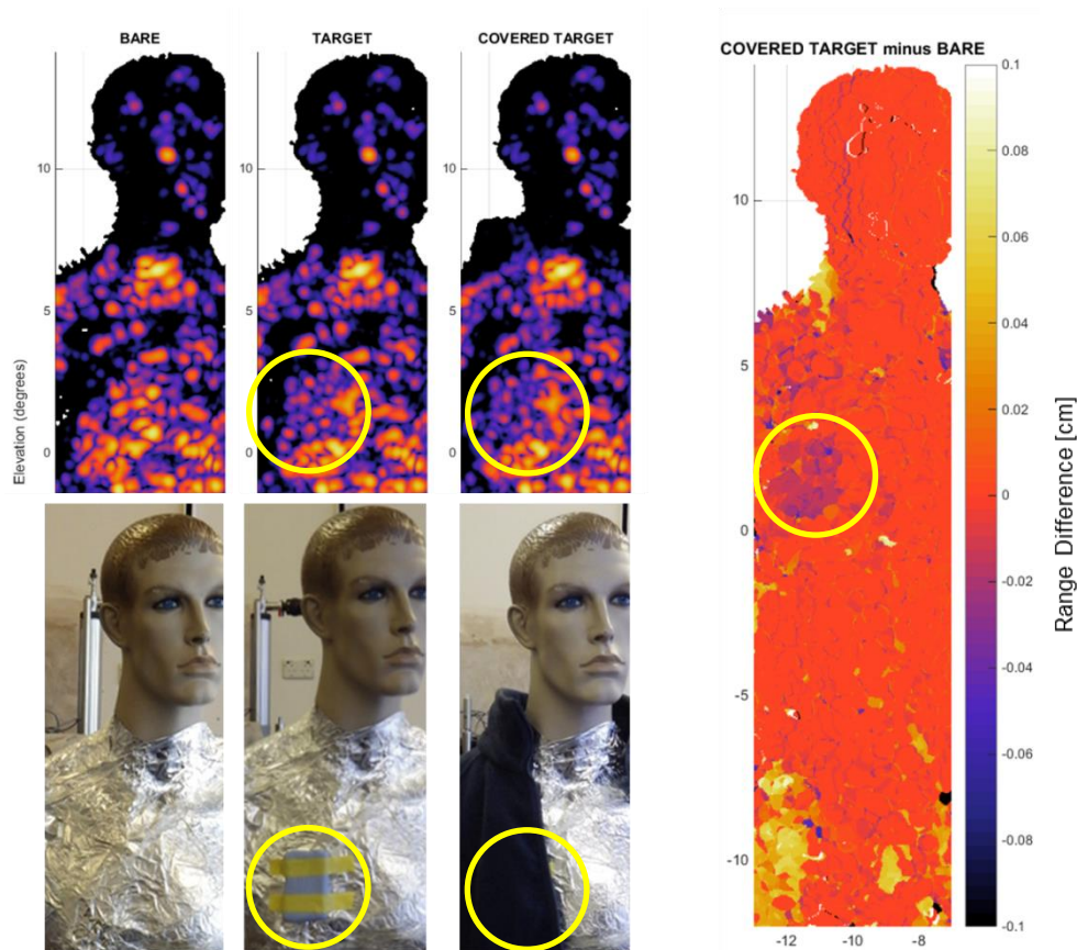
Figure 8. Intensity images of mannequin test subject: bare, with 10 x 6 x 2 cm Blu-Tack target, target covered with fleece (left), range difference image showing depth discrimination of 2 cm thick dielectric concealed target (right).
