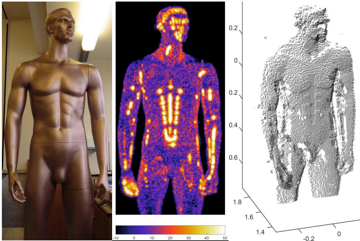
Figure 7. Mannequin test subject (left), 220 GHz radar intensity image (middle) and 3D radar point cloud (right).
