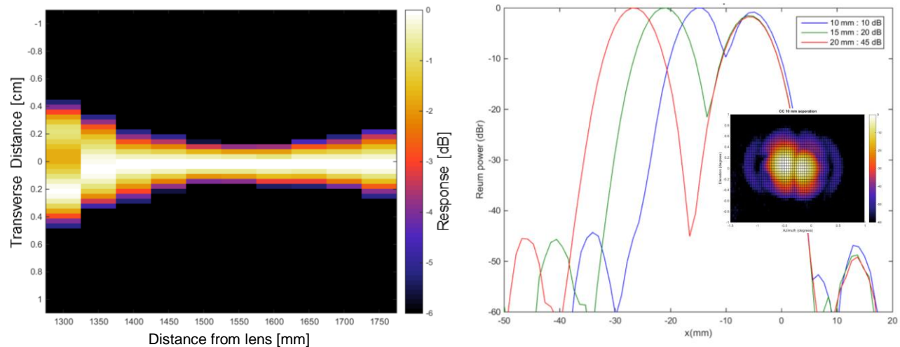
Figure 5. Beam diffraction showing focus at 1550 mm from lens (left) and transverse cuts for two-target separation test showing 20, 15 and 10 mm separations plus radar image of two point targets separated by 10 mm, inset, (right).
