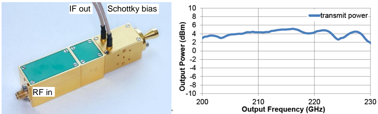
Figure 3. Frequency multiplier chain (x4-x3-x2mix) including self-mixing multiplier final stage (left) and output power versus frequency over 30 GHz bandwidth (right).
