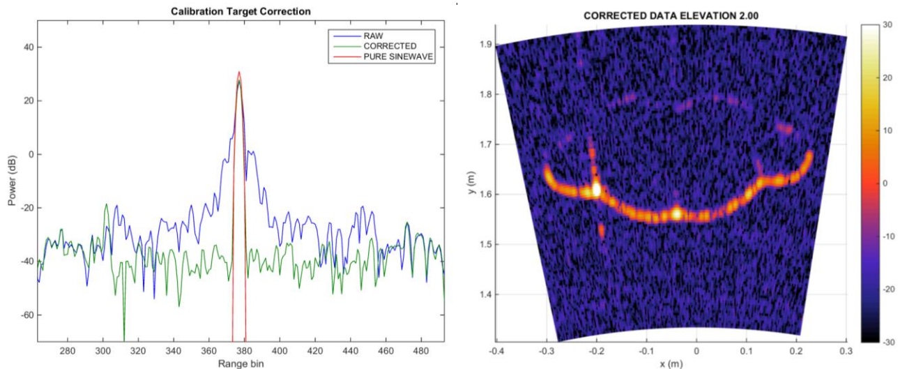
Figure 6. Raw and corrected point responses compared with Fourier transform limited sinewave (left) and azimuth slice through mannequin highlighting range resolution and exhibiting residual phase noise from specular reflections (right).
