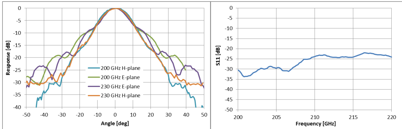
Figure 4. Conical feedhorn measured far-field antenna patterns at 200 and 230 GHz (left) and input port return loss (right).
