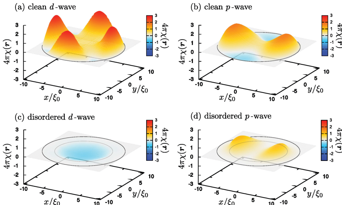
FIG. 2. (Color) Local susceptibilities of small superconducting disks. The results for a d -wave and those for a p -wave superconductor with a clean surface (i.e., w = 0 , \xi/\ell = 0 ) are presented in (a) and (b), respectively. The results for a d -wave and those for a p -wave superconductor with a rough surface ( w = 3\xi_0 , \xi_0/\ell = 1.0 ) are demonstrated in (c) and (d), respectively. The parameters used in the simulation are R = 10\xi_0 , \lambda_L = 5\xi_0 , \omega_c = 10\Delta_0 , H^{\text{ext}} = 0.01 H_{c1} , and T = 0.1 T_c .
