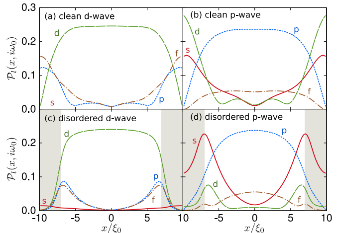
FIG. 5. (Color online) Spatial dependencies of the decomposed pairing functions at the lowest Matsubara frequency on the x axis for (a) a clean d -wave, (b) a clean p -wave, (c) a disordered d -wave, and (d) a disordered p -wave disk. The parameters are set to the same values as those in Fig. 2. The shadowed areas indicate the disordered regions.
