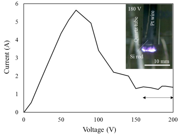
Figure 2. (color online) Current–voltage curve in 0.1 M HCl solution. Above 150 V, plasma generation with light emission occurred and the intensity of the light emission increased with increases in voltage. The inset shows a photograph of the electrode at 180 V.
