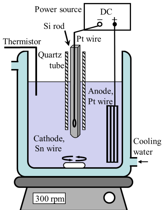
Figure 1. (color online) Experimental setup for producing Si particles. A Si rod electrode was placed in a glass cell with a cooling jacket, in which the upper part of the Si rod was shielded by a quartz glass tube to generate plasma at the bottom tip of the electrode.
