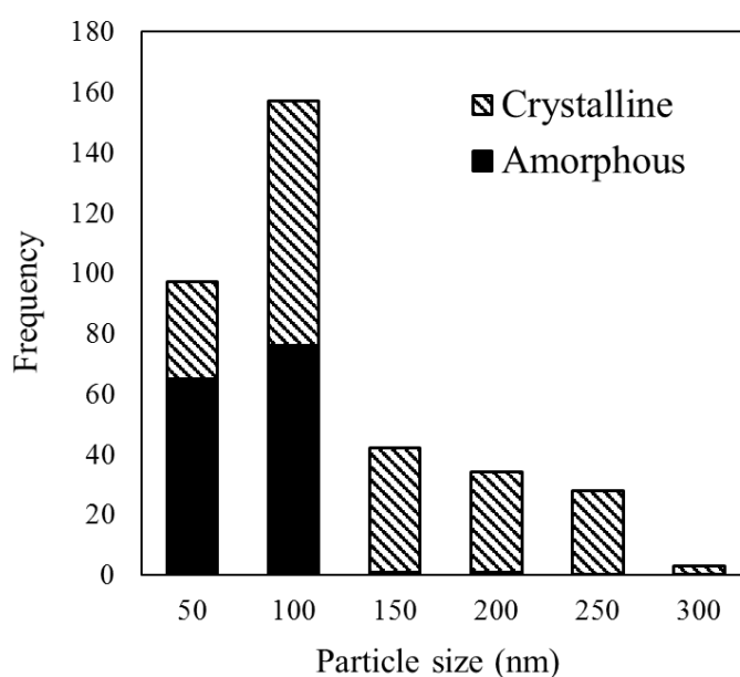
Figure 9. Size distribution of particles obtained by plasma electrolysis in 0.1 M HNO 3 at an applied voltage of 140 V. The 363 particles were analysed by TEM to distinguish the crystal structures.
