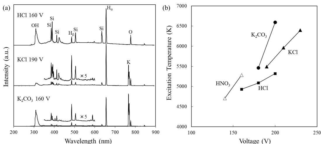
Figure 3. (a) Spectra of the electrode in different electrolytes. (b) Excitation temperature versus applied voltage in different electrolytes. The excitation temperatures were calculated from the intensity of the light emission of H α (656.3 nm) and H β (486.1 nm) when the electrons were assumed to have a Boltzmann distribution.
