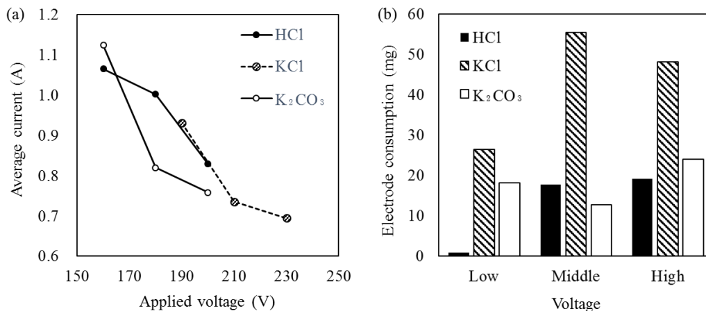
Figure 5 (a) Relationship between the applied voltage and average current for different electrolytes. (b) Electrode consumption at different conditions.
