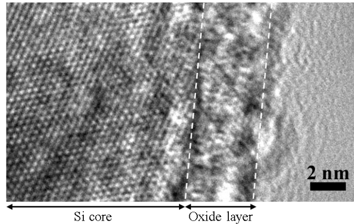
Figure 7. Enlarged TEM image of Si-NP produced in HNO 3 solution. The oxide layer with a thickness of 3–4 nm was formed on the Si surface.
