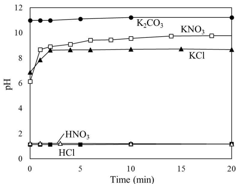
Figure 8. Changes in pH values during plasma electrolysis in different electrolytes. When the neutral solutions of KNO 3 and KCl were used, the pH value was increased owing to the consumption of Cl - and KNO 3 - ions.
