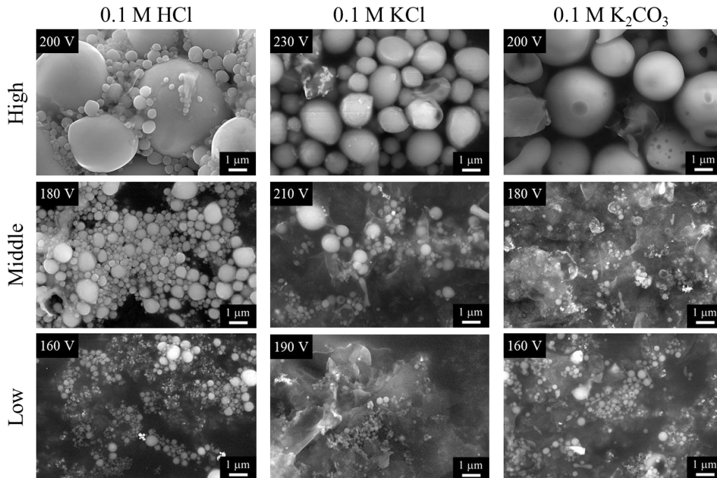
Figure 4. SEM image of Si particles produced in different electrolytes at different applied voltages.
