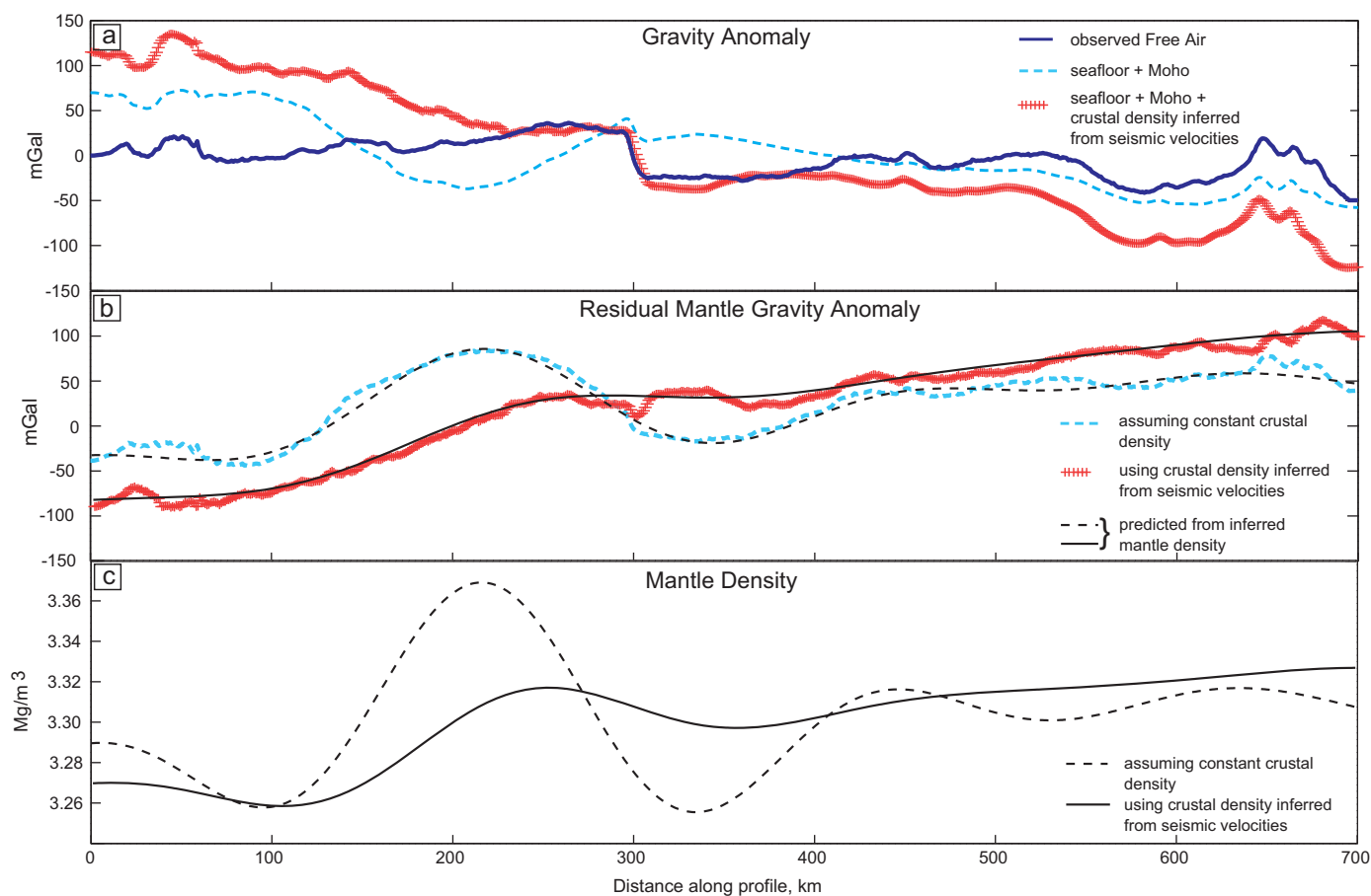
Figure 5. (a) Free air gravity anomaly and predicted gravity anomalies, (b) residual mantle gravity anomaly, and (c) mantle density plotted as a function of distance along the profile. (a) The observed Free Air Gravity anomaly (blue solid line) is compared to the predicted gravity anomaly for the seafloor and Moho topography using constant crustal density (dashed light blue line) and variations in crustal density inferred from seismic velocity variations (red crosses); see text for discussion. (b) The residual mantle gravity anomaly is calculated by subtracting the predicted gravity anomaly due to the crustal structure shown in Figure 5a from the observed Free Air anomaly both for constant and varying crustal density; same line styles as in Figure 5a. Figure 5c Mantle density anomalies are calculated by downward continuation of the residual mantle gravity anomaly using a compensation depth of 100 km and a band-pass filter from 150 to 1000 km for both constant crustal density (dashed line) and varying crustal density (solid line). The component of the residual mantle gravity anomaly that is accounted for by the mantle densities variations inferred in Figure 5c is also shown in Figure 5b (solid and dashed black lines). Note the gradual decrease in mantle density toward Iceland in the west.
