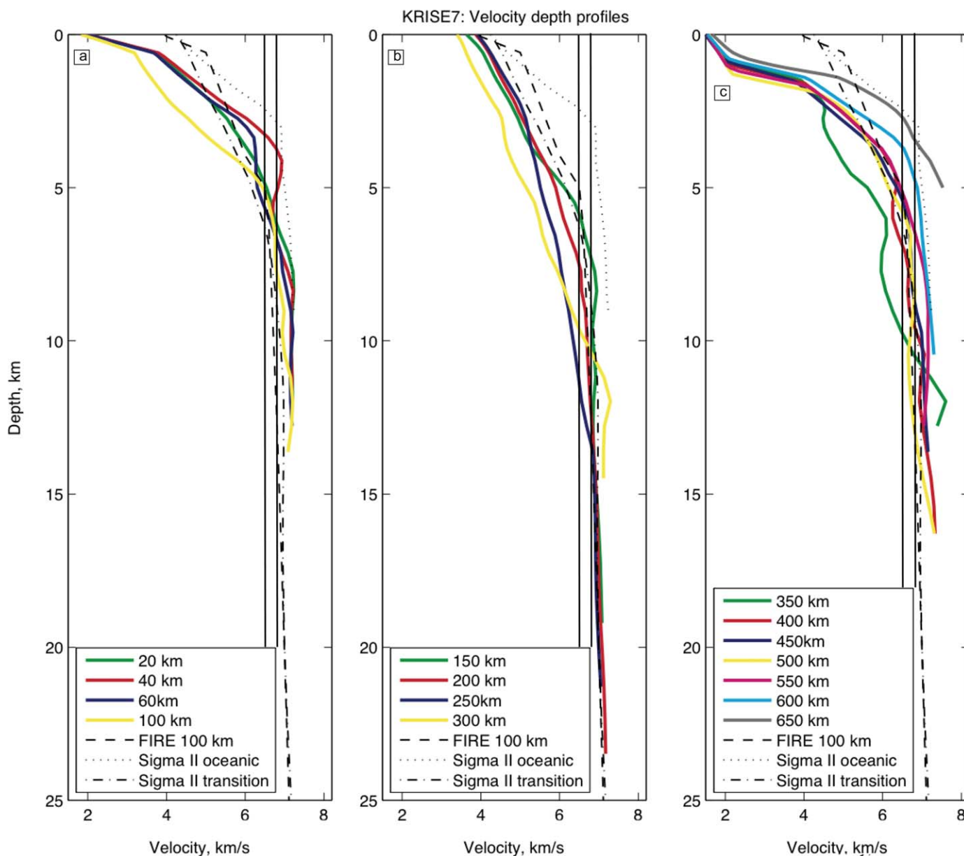
Figure 6. Plots of 1-D velocity-depth profiles averaged over 20–50 km sections of the KRISE7 transect (Figure 4), color coded by distance. Average 1-D velocity structure of the FIRE profile in E-Iceland [Staples et al. , 1997] and Sigma II profile along the SE-Greenland margin [Korenaga et al. , 2000, 2001] are shown for comparison. Vertical lines are at 6.5 and 6.8 km/s. Note similarities in crustal velocities below 10 km depth.
