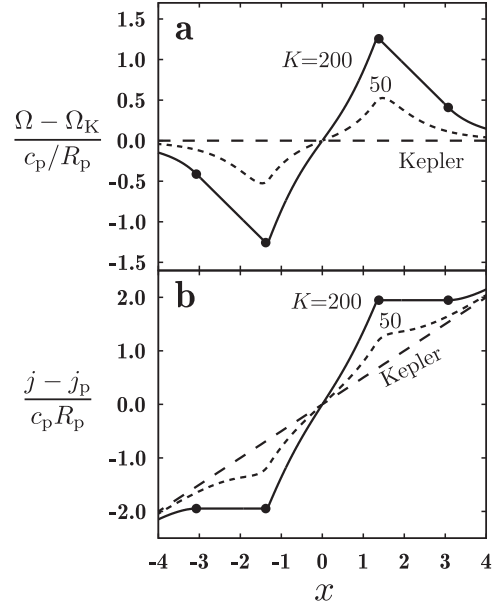
Figure 3. (a) Deviation from Keplerian disc rotation and (b) specific angular momenta, for K = 50 (dashed) and 200 (solid). The filled circles indicate the edge of the marginally stable region for the Rayleigh condition.
