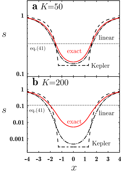
Figure 2. Surface density distributions for K = 50 (a) and 200 (b). The red line is the exact solution (see text). The chain line is the linear solution given by equation (43) and the dashed line is the solution for the Keplerian case (equation 37). The dotted line represents the minimum surface densities for the wide-limit gap given by equation (41).
