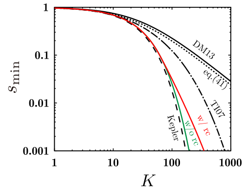
Figure 8. Minimum surface densities, s_{\min} , for the exact solution (red line) and the solution without the Rayleigh condition (green line). The dashed line is s_{\min} in the Keplerian case. The chain, dotted and solid lines denote s_{\min} given by the model of TI07 , the wide-limit gap (equation 41) and the empirical relation of DM13 (equation 42), respectively.
