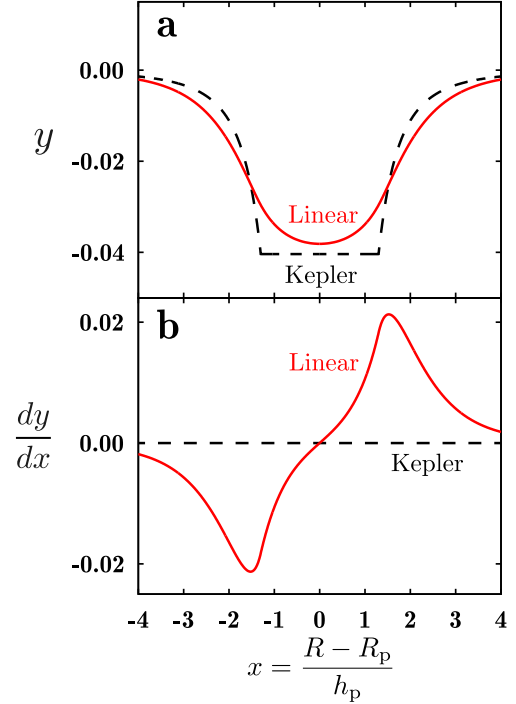
Figure 1. Linear solution for y (a) and dy/dx (b). The surface density and angular velocity are given by y and dy/dx with equations (43) and (45), respectively. The dashed line is the solution for the Keplerian disc.
