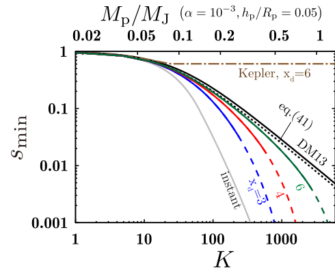
Figure 12. Minimum surface densities, s_{\min} , of the exact solutions in the case with the wave propagation for x_d = 3 (blue), 4 (red) and 6 (green). The parameter w_d is h_p . We also plot results by DM13 (equation 42, solid line) and the wide-limit gap (equation 41, dotted line) and the exact solution with instantaneous damping (grey line). The dashed lines indicate exact solutions with unrealistic wave propagation.
