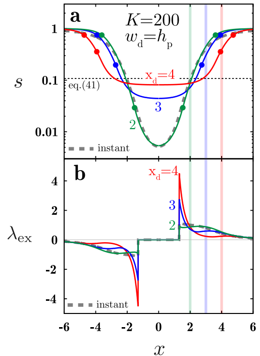
Figure 9. Surface densities (a) and excitation torque densities (b) in the case with the wave propagation for K = 200 . The green, blue and red lines denote the solutions with x_d = 2, 3 and 4, respectively. The parameter w_d is set to h_p . The grey dashed line is the surface density in the case with instantaneous wave damping. The dotted line in (a) represents the minimum surface density for the wide-limit gap given by equation (41), i.e. s_{\min} = 0.109 .
