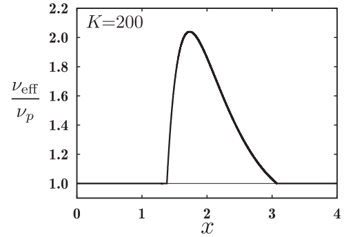
Figure 7. Effective viscosity \nu_{\text{eff}} of the exact solution with K = 200 .
