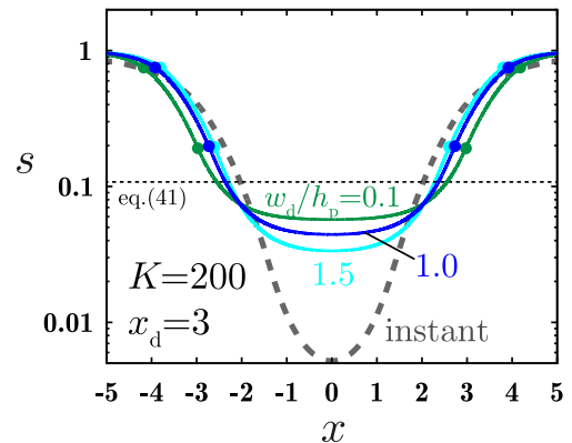
Figure 10. Gap structures for w_d = 0.1h_p (green), h_p (blue) and 1.5h_p (light-blue). The parameters K and x_d are set to 200 and 3, respectively. The grey dashed line indicates the solution in the instantaneous damping case and the dotted line is the minimum surface density of the wide-limit gap (equation 41).
