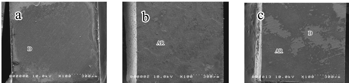
Fig. 2 Field-emission scanning electron micrographs of de-bonded samples show their fractured surfaces. (a) adhesive; (b) cohesive; (c) mixed. Abbreviations: adhesive resin (AR) ; dentin (D).
